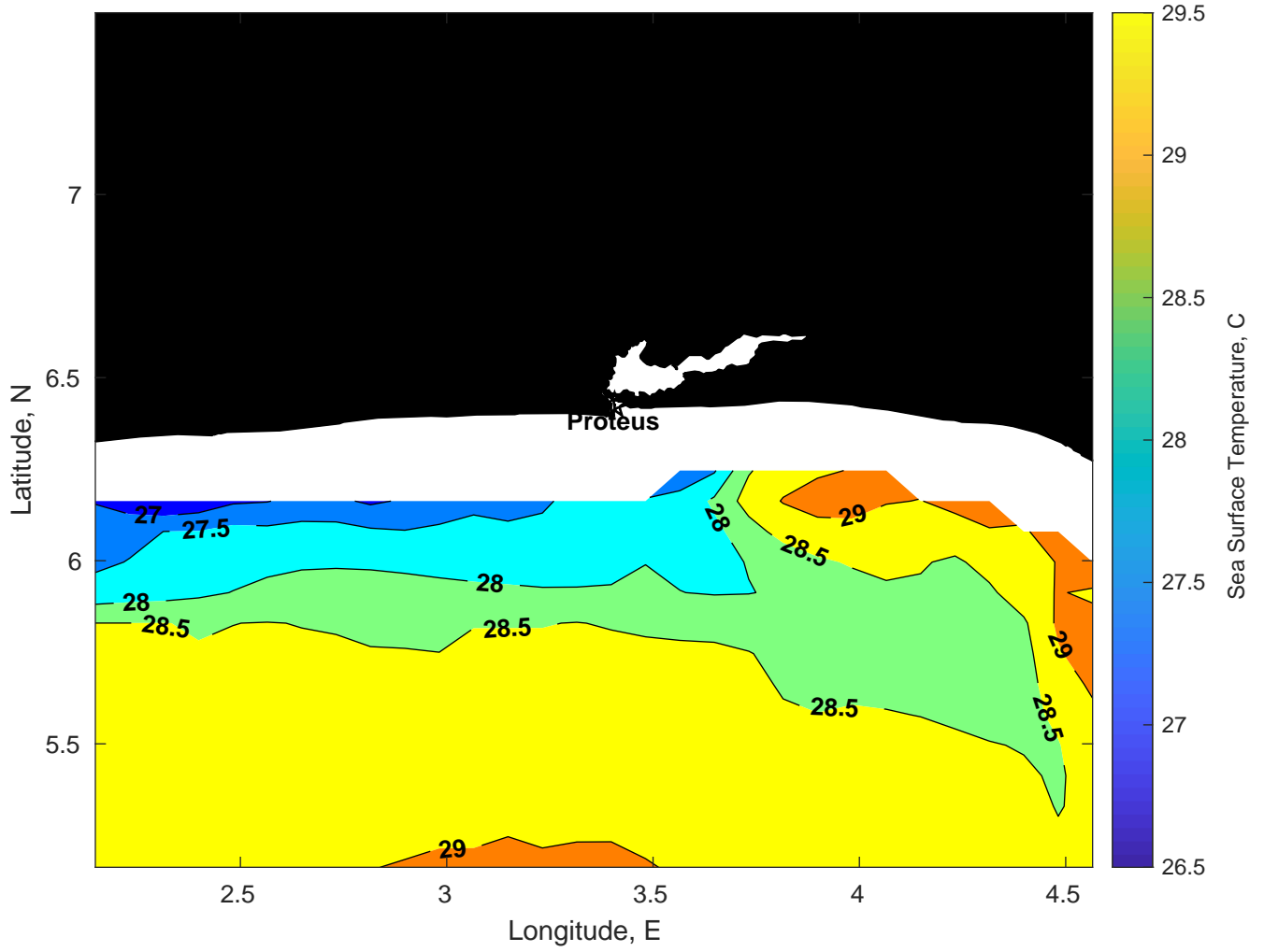
SST for Proteus at 04-Mar-2025 00:00:00
