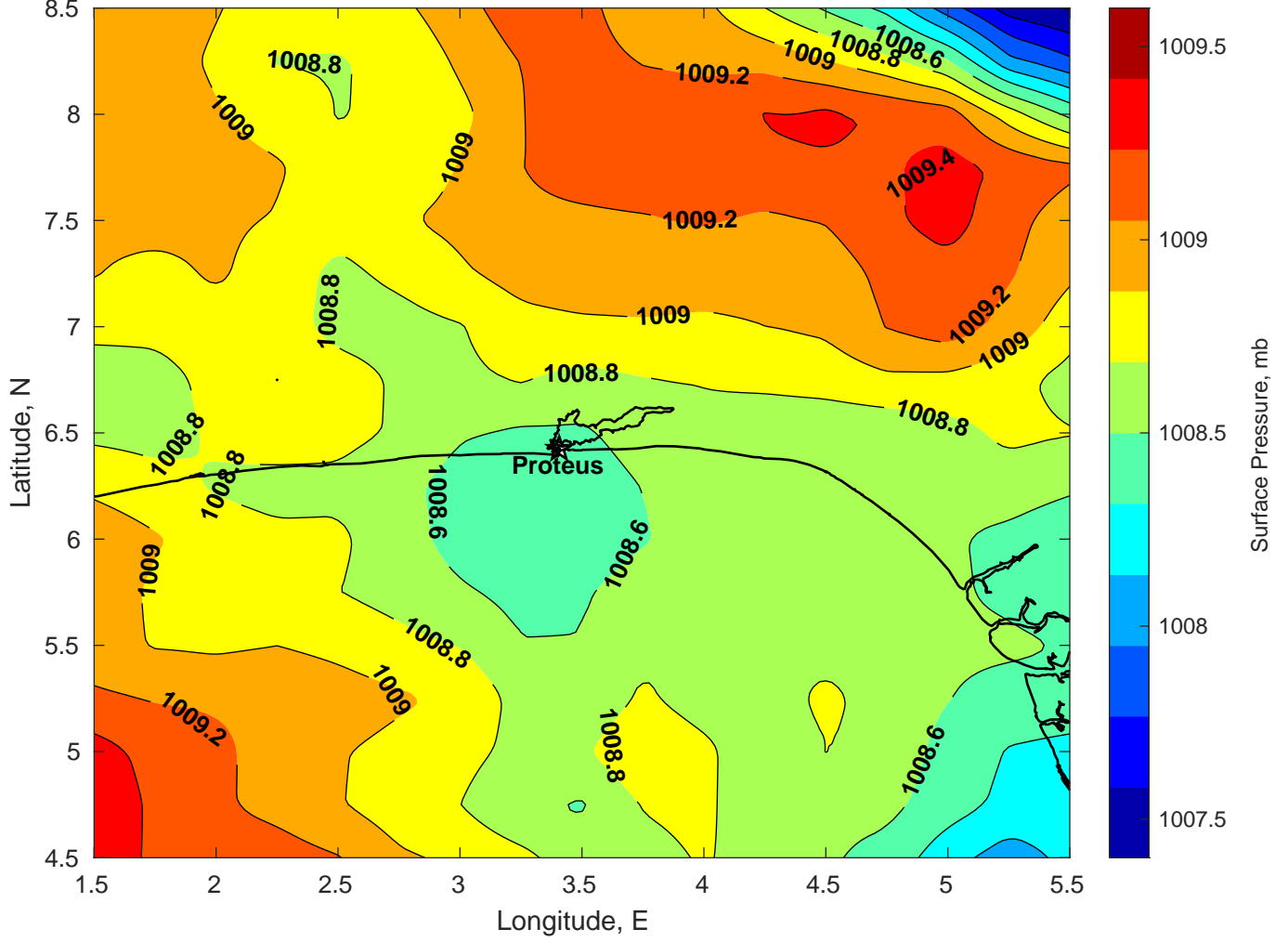
Surface Pressure (mb) for Proteus at 06-Mar-2025 00:00:00
