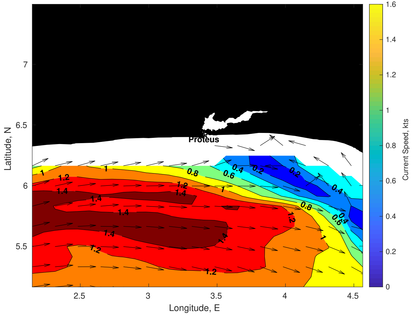
Surface Currents for Proteus at 04-Mar-2025 00:00:00
