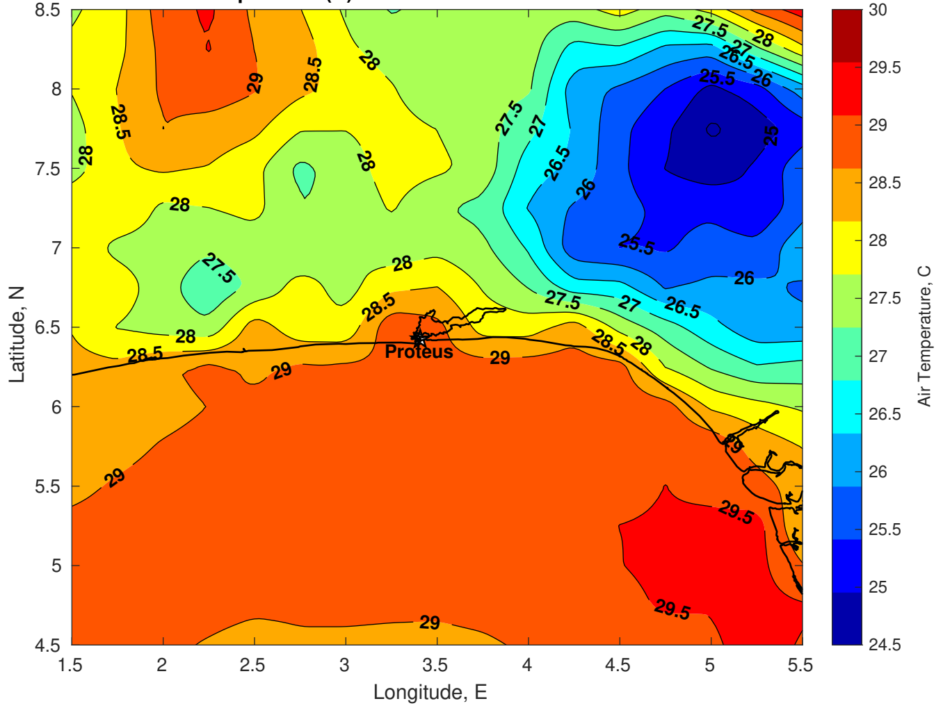
Air Temperature (C) for Proteus at 05-Mar-2025
