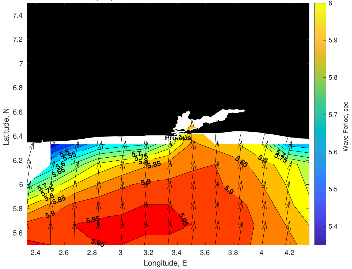
Wave Period (sec) for Proteus at 05-Mar-2025 09:00:00
