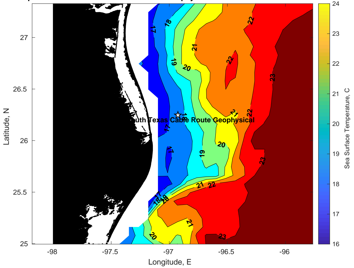
SST for Tampnet P2378 South Texas Cable Route Geophysical at 04-Mar-2025 00:00:00
