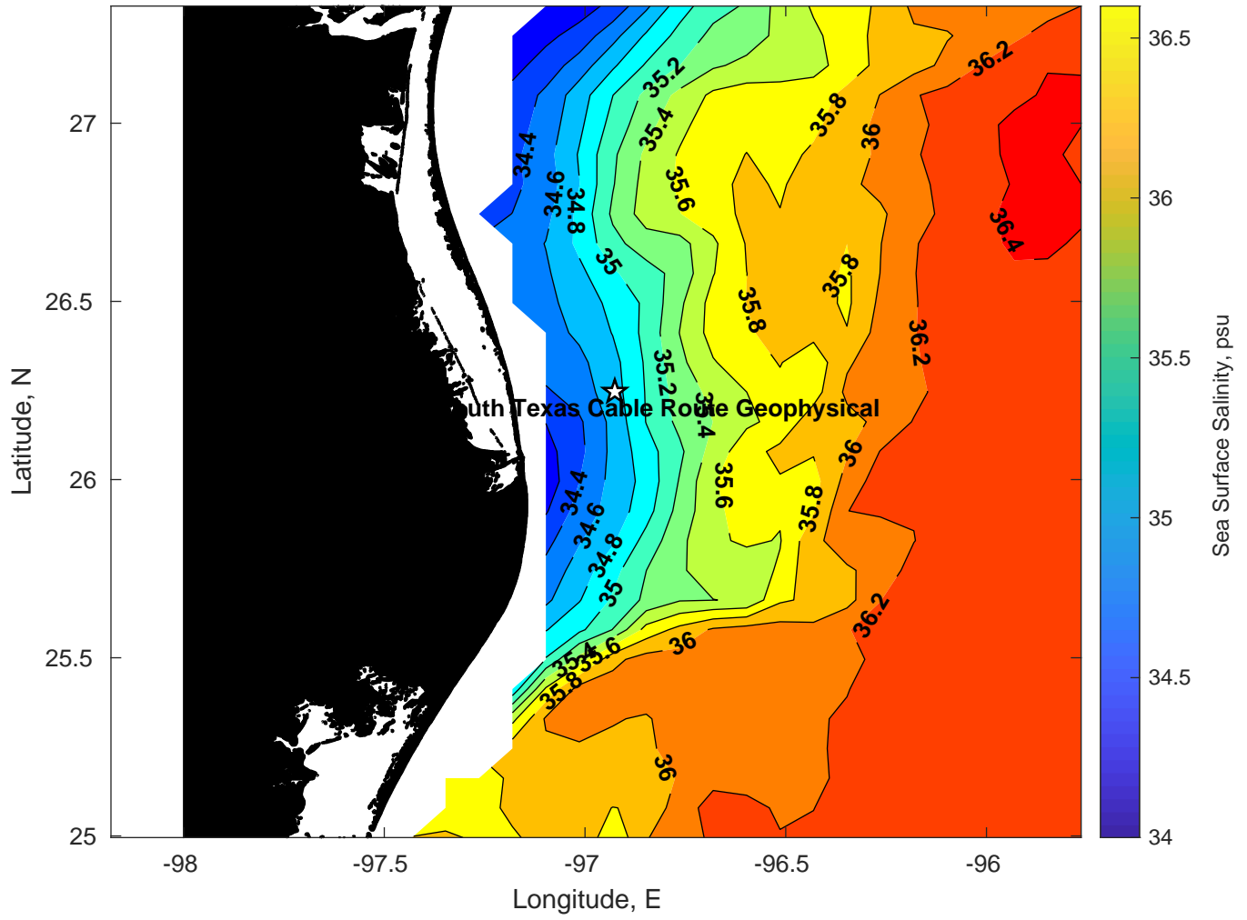
Surface Salinity for Tampnet P2378 South Texas Cable Route Geophysical at 04-Mar-2025 00:00:00
