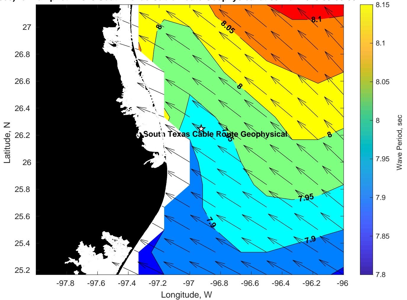
Period (sec) for Tampnet P2378 South Texas Cable Route Geophysical at 05-Mar-2025 09:00:00
