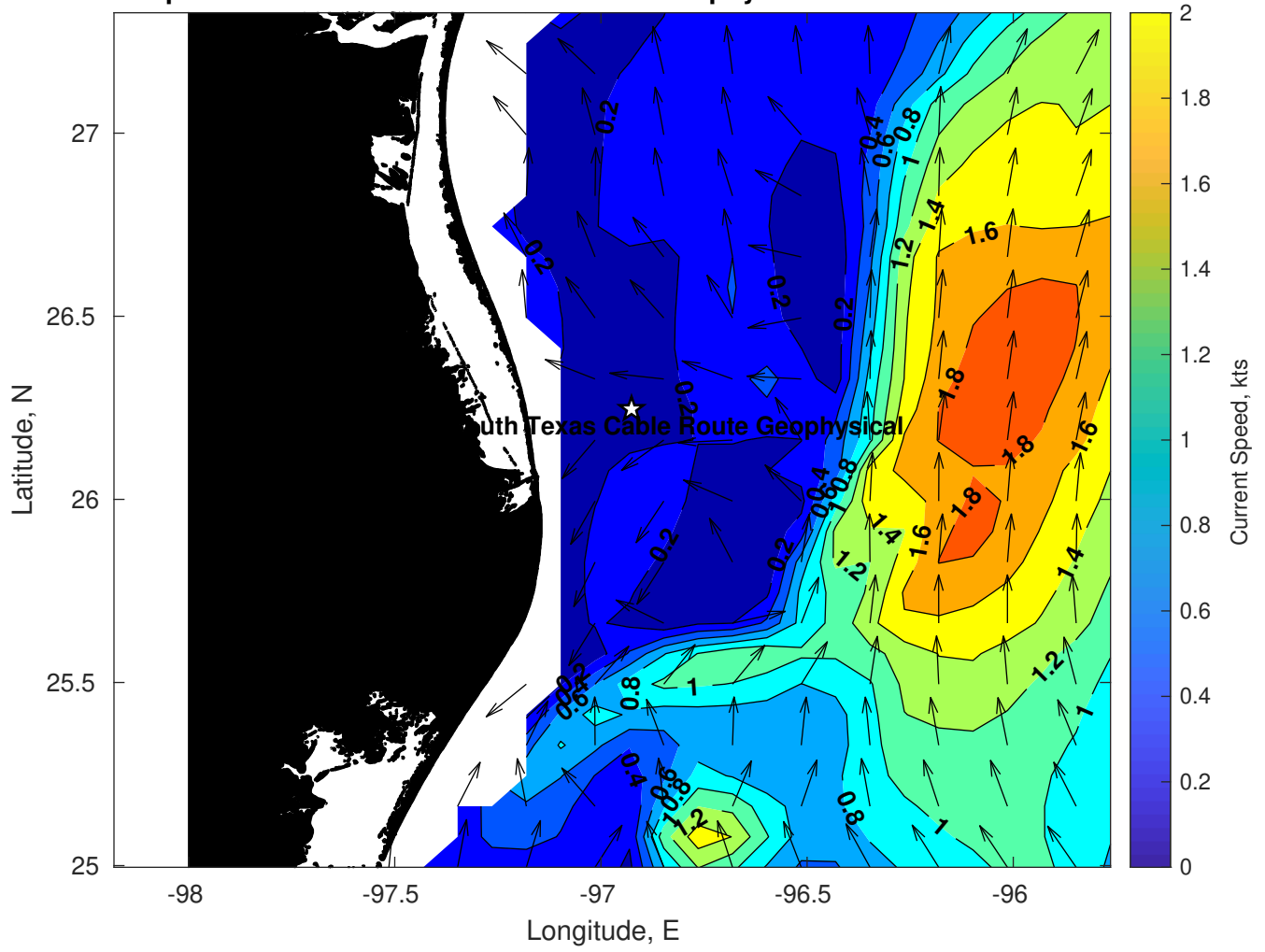
Surface Currents for Tampnet P2378 South Texas Cable Route Geophysical at 04-Mar-2025 00:00:00
