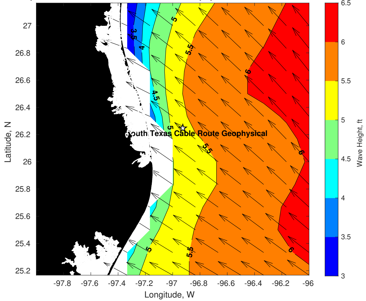
Wave Height (ft) for Tampnet P2378 South Texas Cable Route Geophysical at 05-Mar-2025 09:00:00
