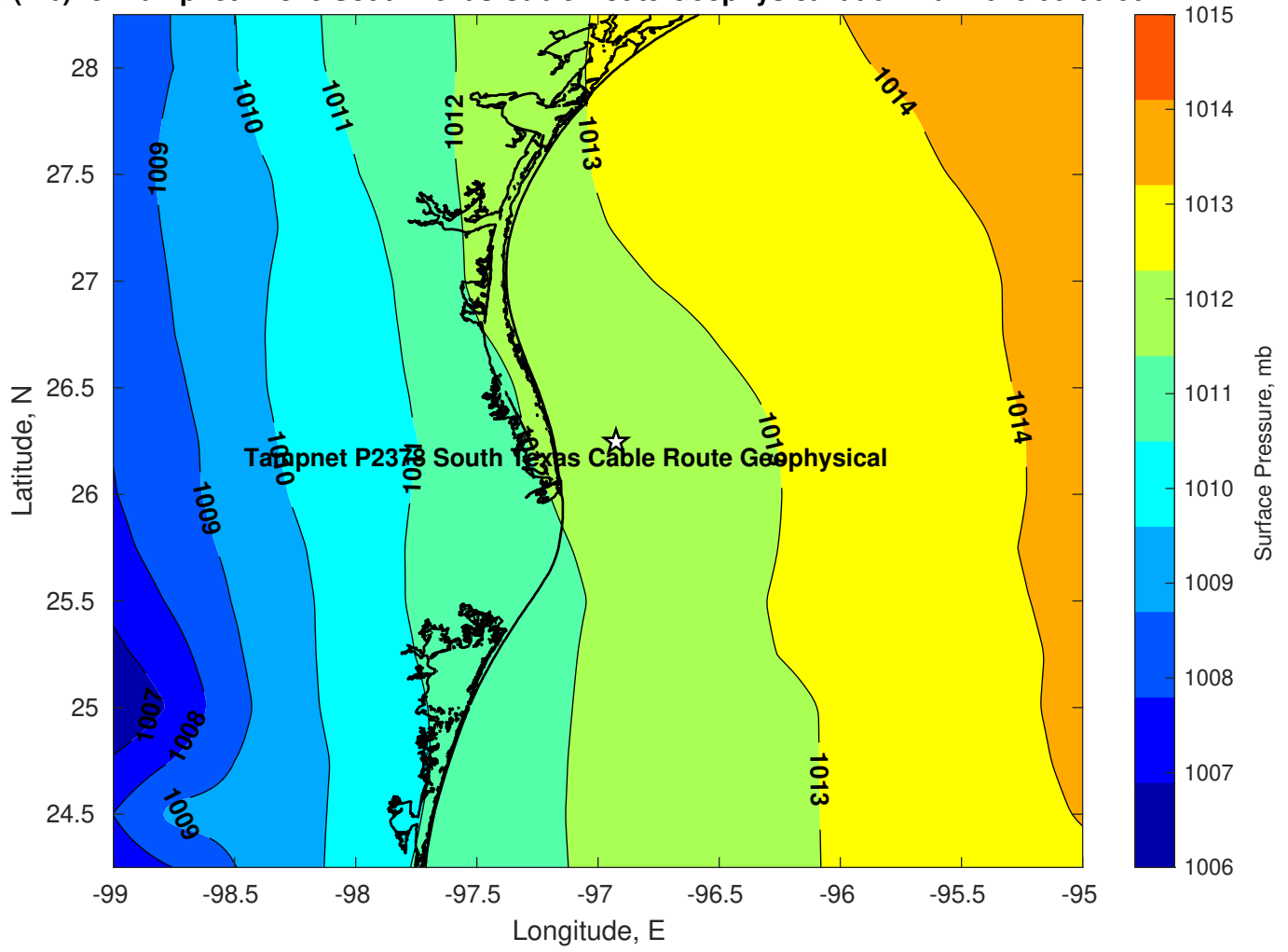
Pressure (mb) for Tampnet P2378 South Texas Cable Route Geophysical at 07-Mar-2025 00:00:00
