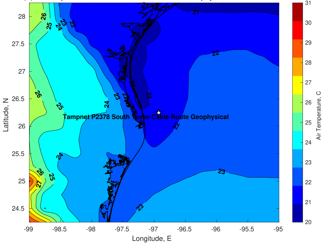
Air Temperature (C) for Tampnet P2378 South Texas Cable Route Geophysical at 05-Mar-2025
