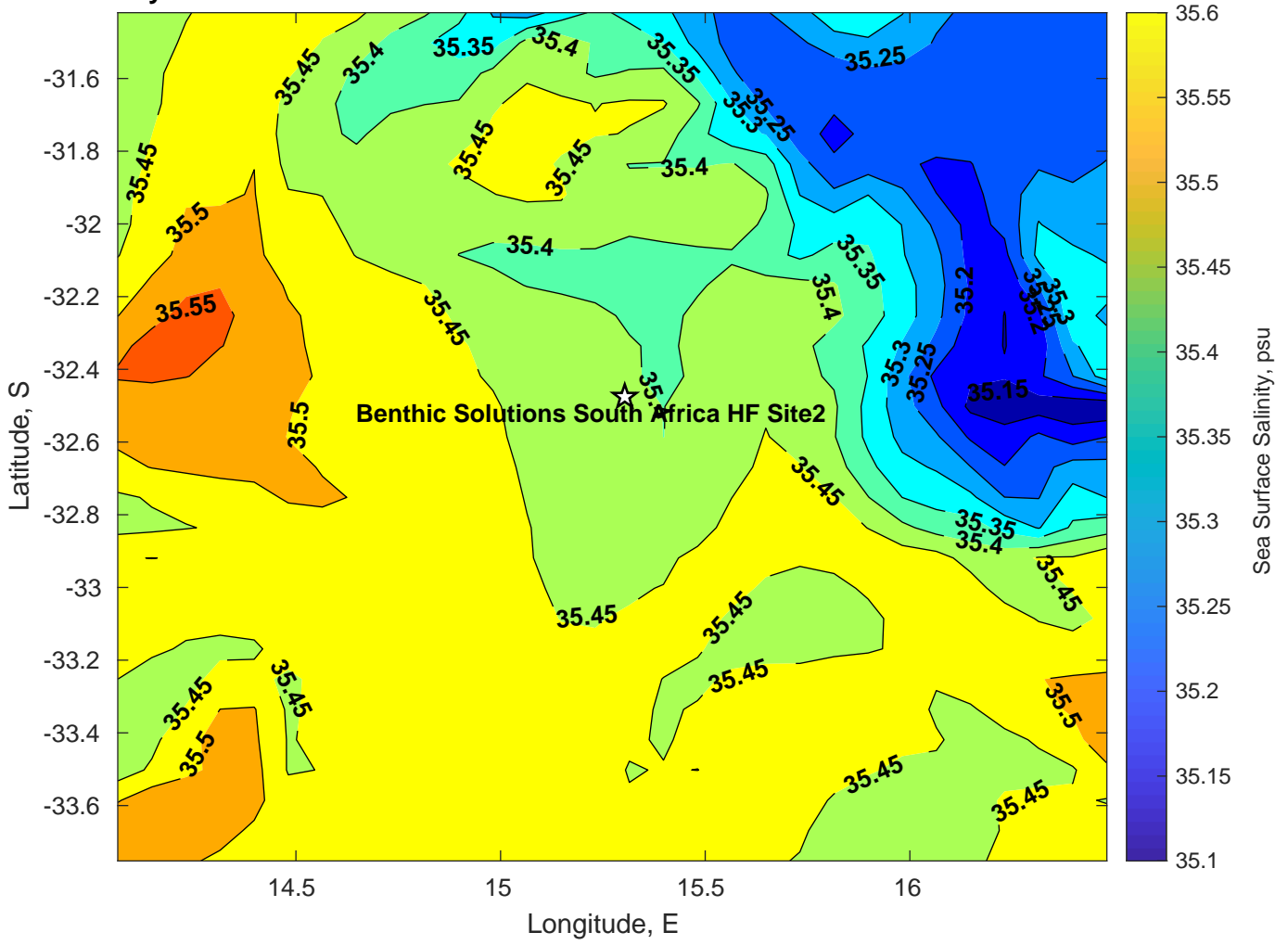
Surface Salinity for Benthic Solutions South Africa HF Site2 at 05-Mar-2025 00:00:00
