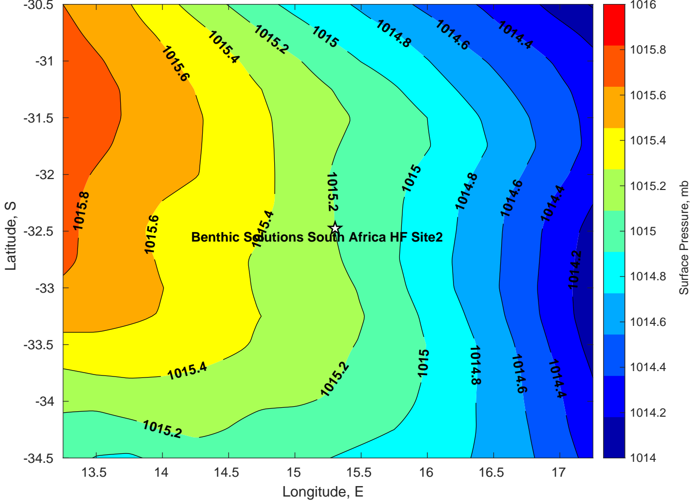
Surface Pressure (mb) for Benthic Solutions South Africa HF Site2 at 06-Mar-2025 00:00:00
