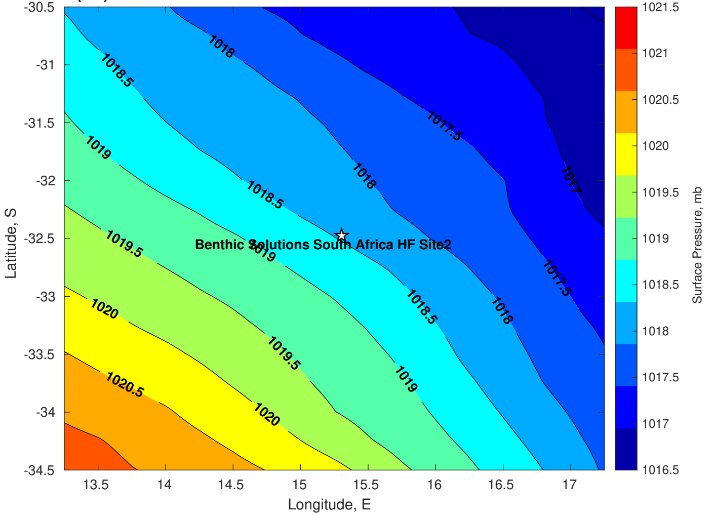
Surface Pressure (mb) for Benthic Solutions South Africa HF Site2 at 07-Mar-2025 00:00:00
