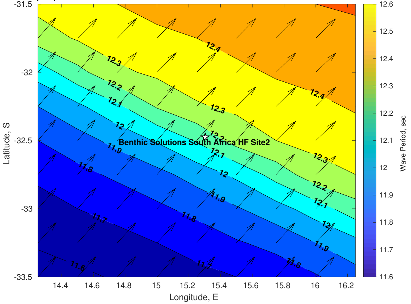
Wave Period (sec) for Benthic Solutions South Africa HF Site2 at 06-Mar-2025 09:00:00
