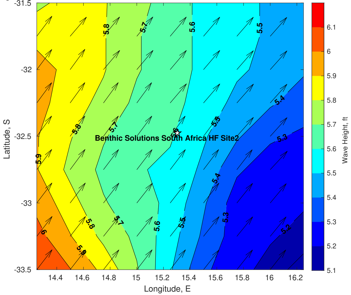
Wave Height (ft) for Benthic Solutions South Africa HF Site2 at 06-Mar-2025 09:00:00
