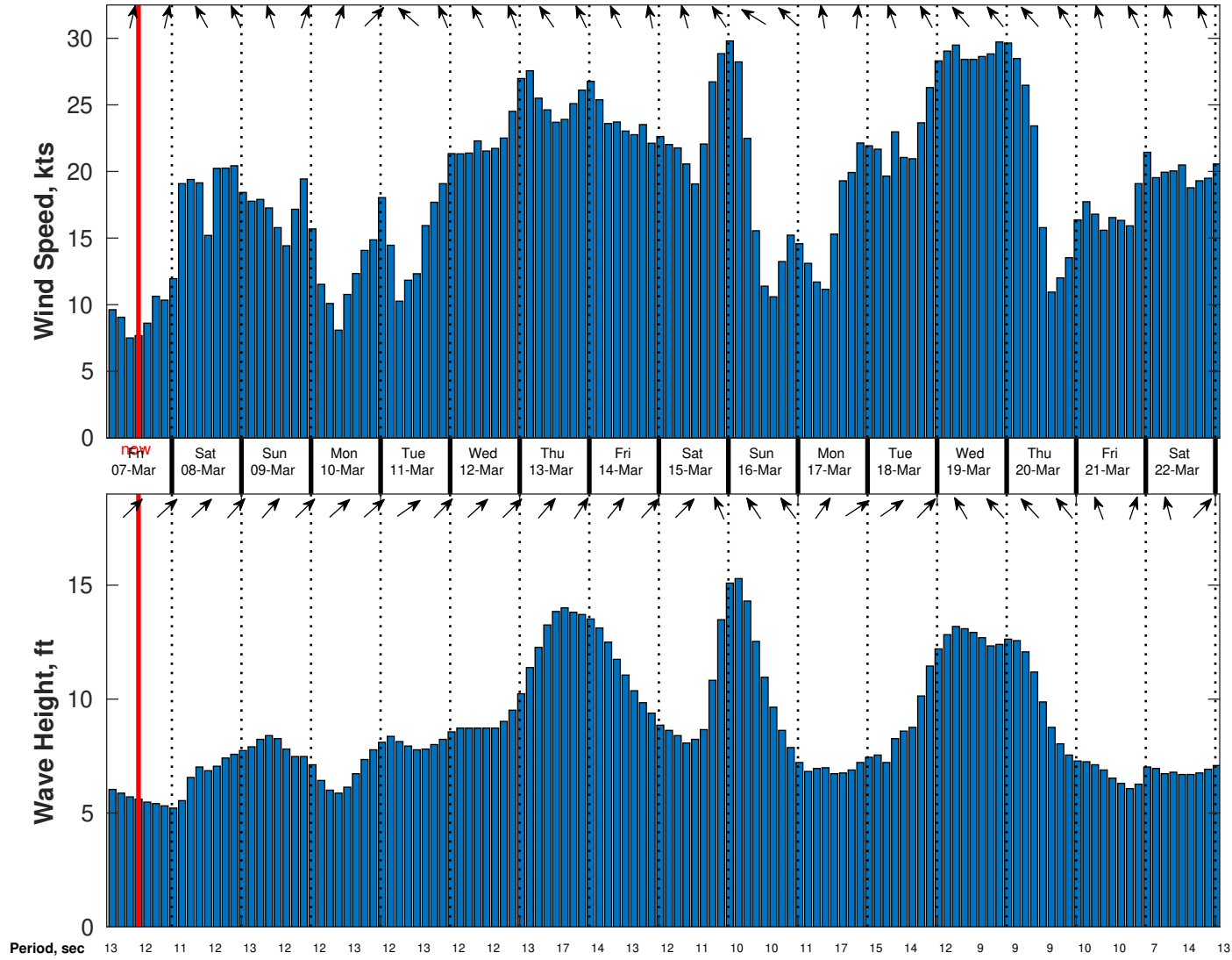
Wind & Wave Forecast for Benthic Solutions South Africa HF Site2 from 06-Mar-2025 02:00:00 to 22-Mar-2025 02:00:00
