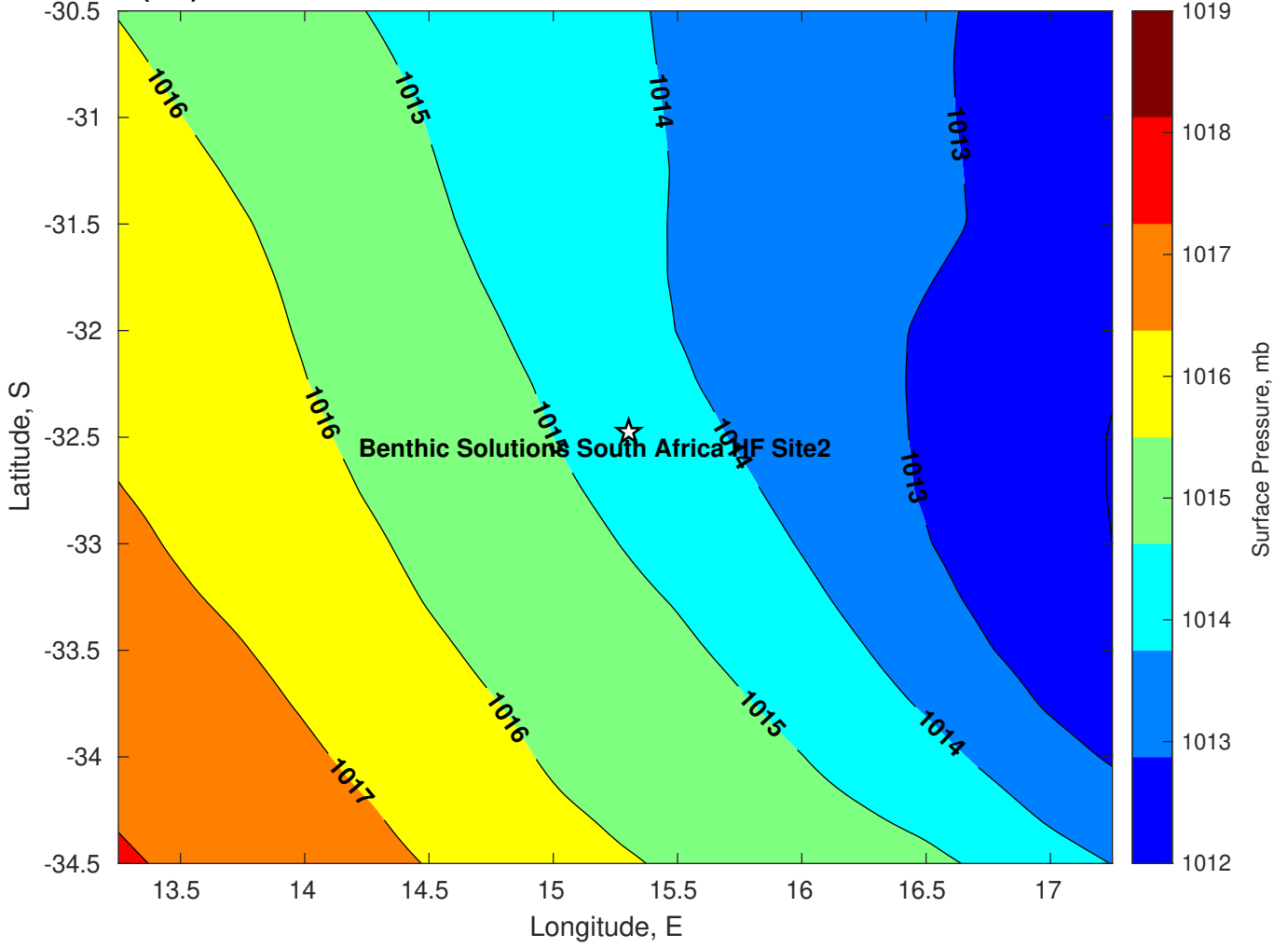
Surface Pressure (mb) for Benthic Solutions South Africa HF Site2 at 08-Mar-2025 00:00:00
