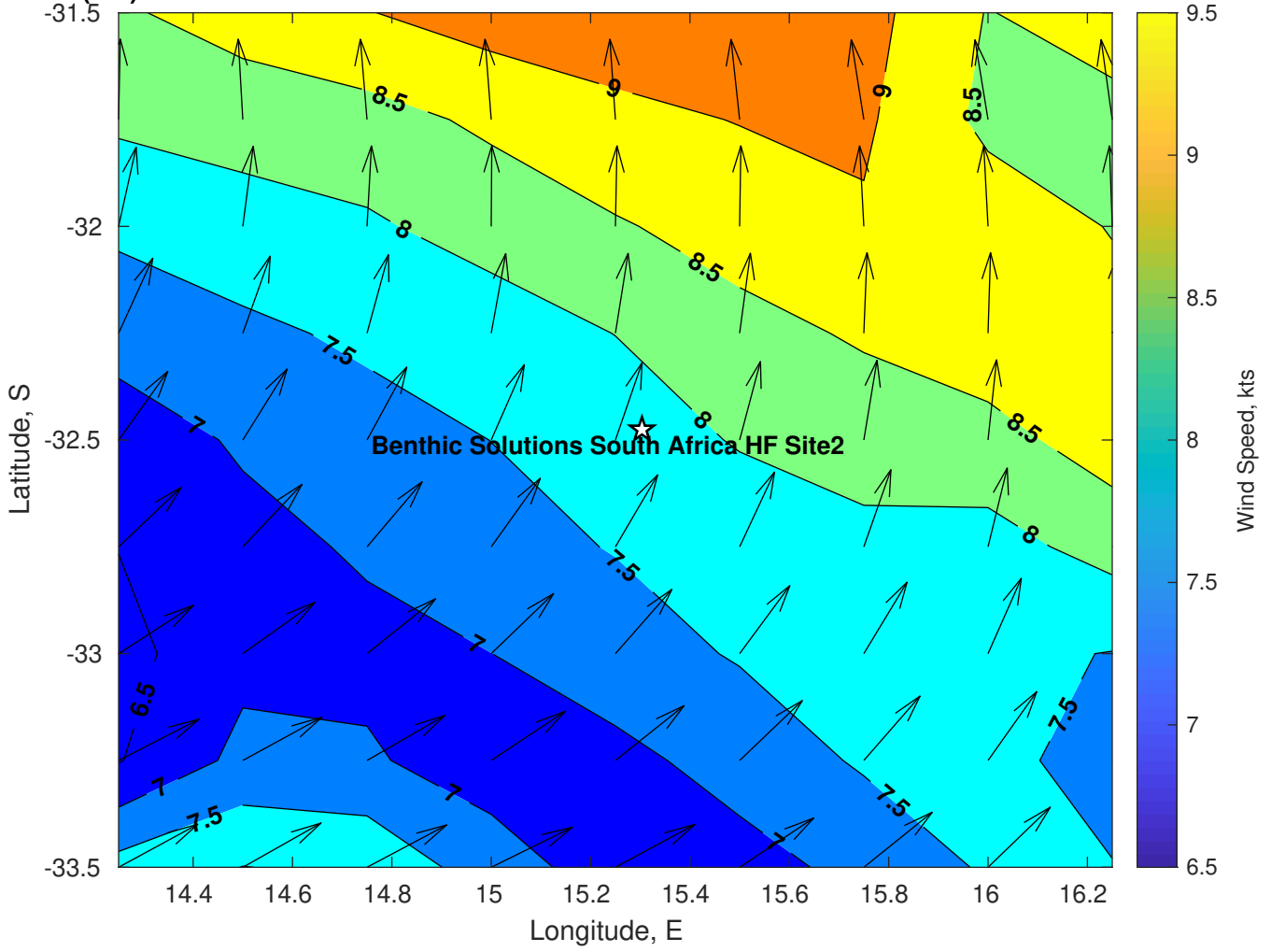
Winds (kts) for Benthic Solutions South Africa HF Site2 at 06-Mar-2025 09:00:00
