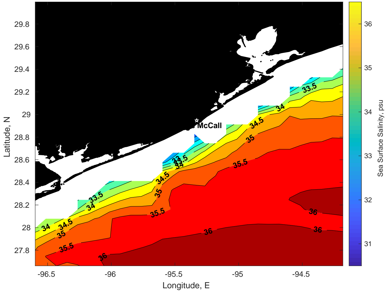
Surface Salinity for Brooks McCall at 05-Mar-2025 00:00:00
