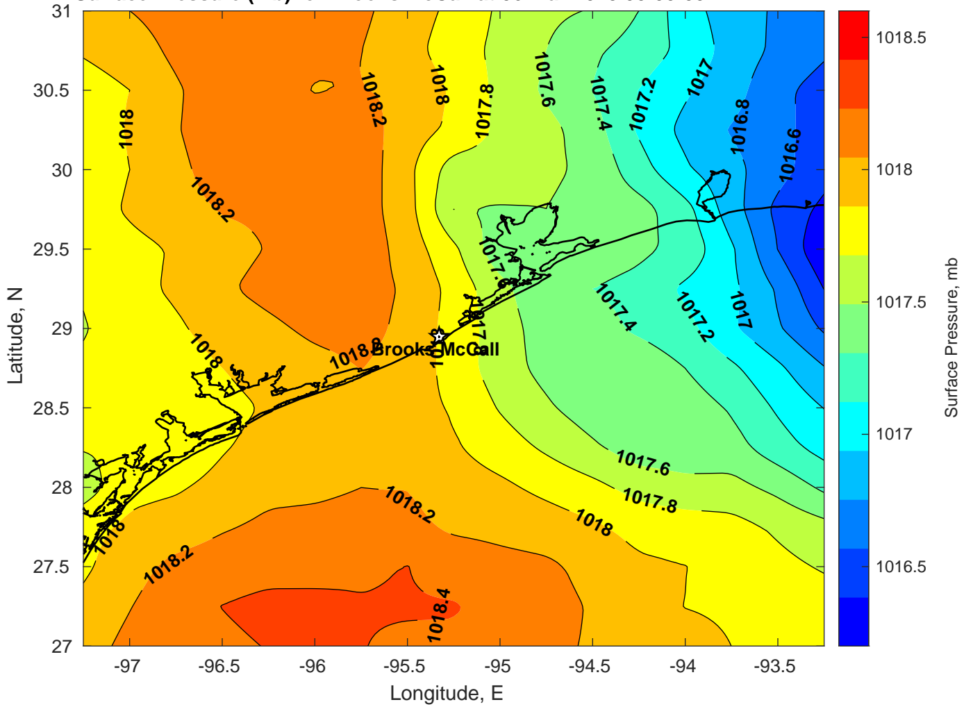
Surface Pressure (mb) for Brooks McCall at 06-Mar-2025 00:00:00
