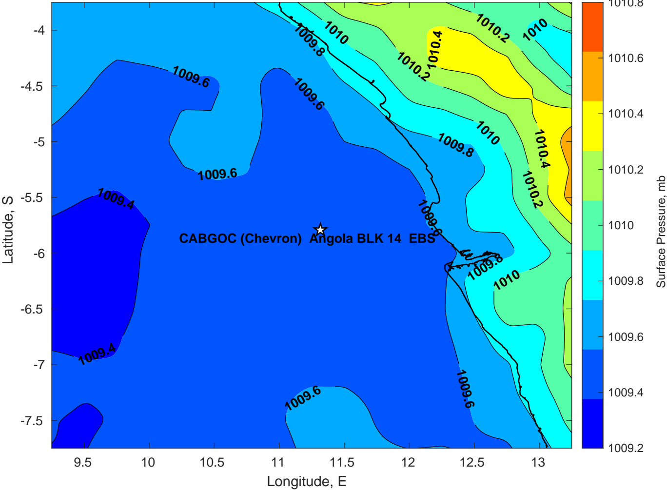
Surface Pressure (mb) for CABGOC (Chevron) Angola BLK 14 EBS at 08-Mar-2025 00:00:00
