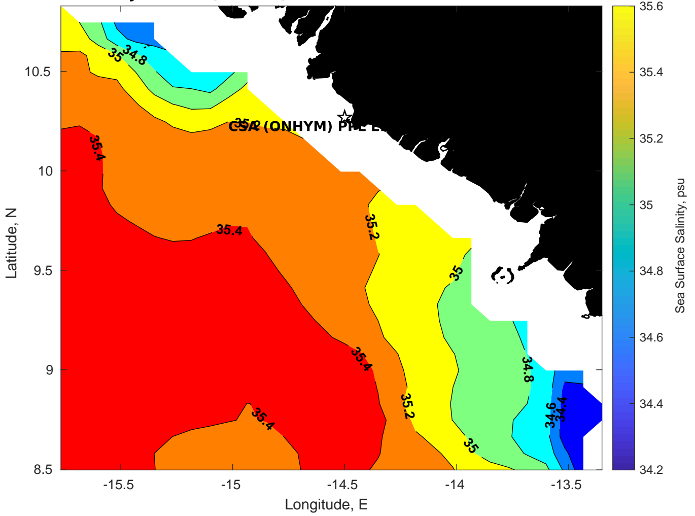
Surface Salinity for CSA (ONHYM) PPL EBS - Guinea at 05-Mar-2025 00:00:00
