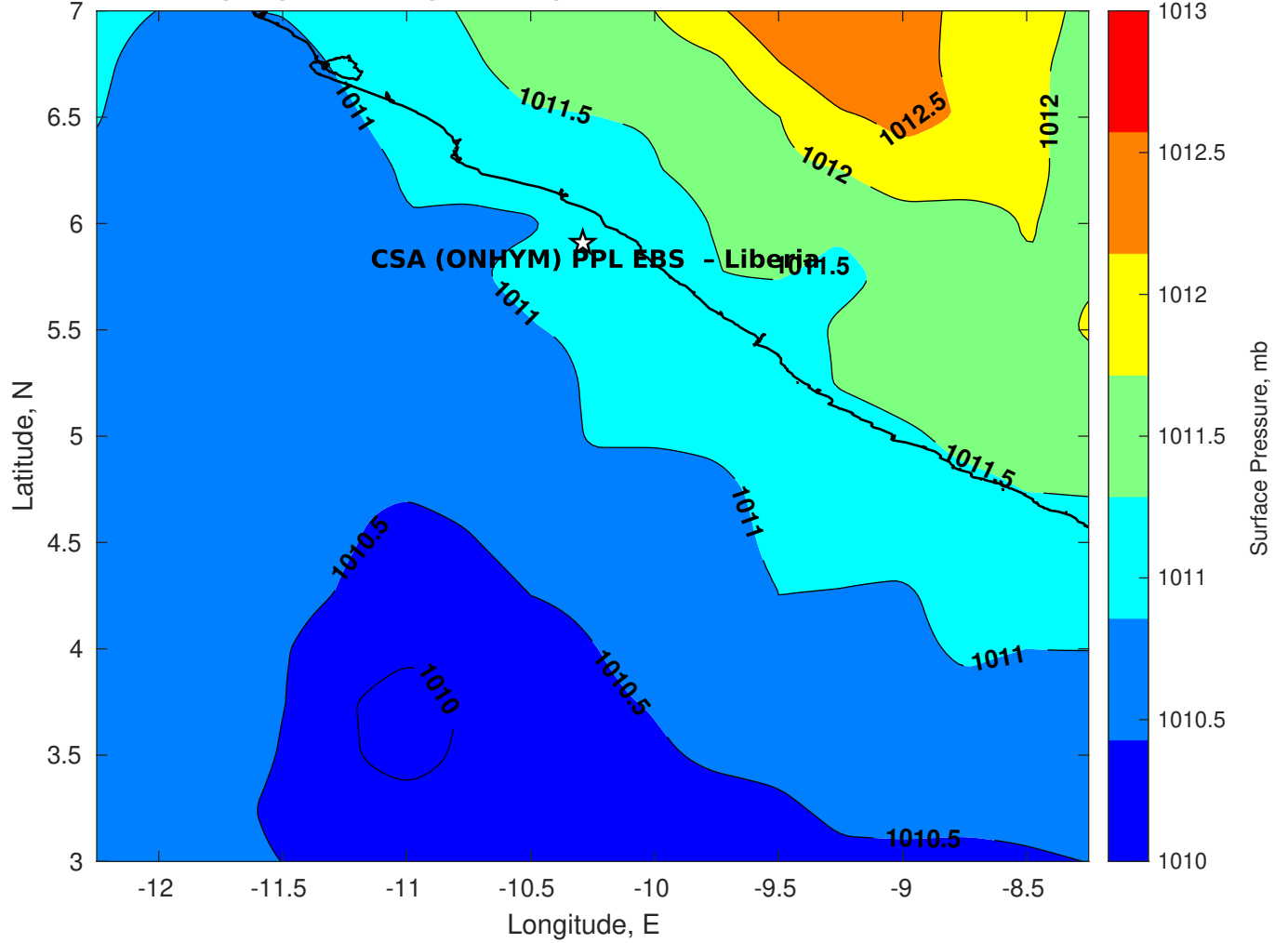
Surface Pressure (mb) for CSA (ONHYM) PPL EBS - Liberia at 06-Mar-2025 00:00:00
