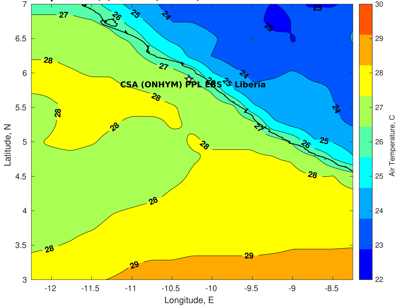
Air Temperature (C) for CSA (ONHYM) PPL EBS - Liberia at 06-Mar-2025
