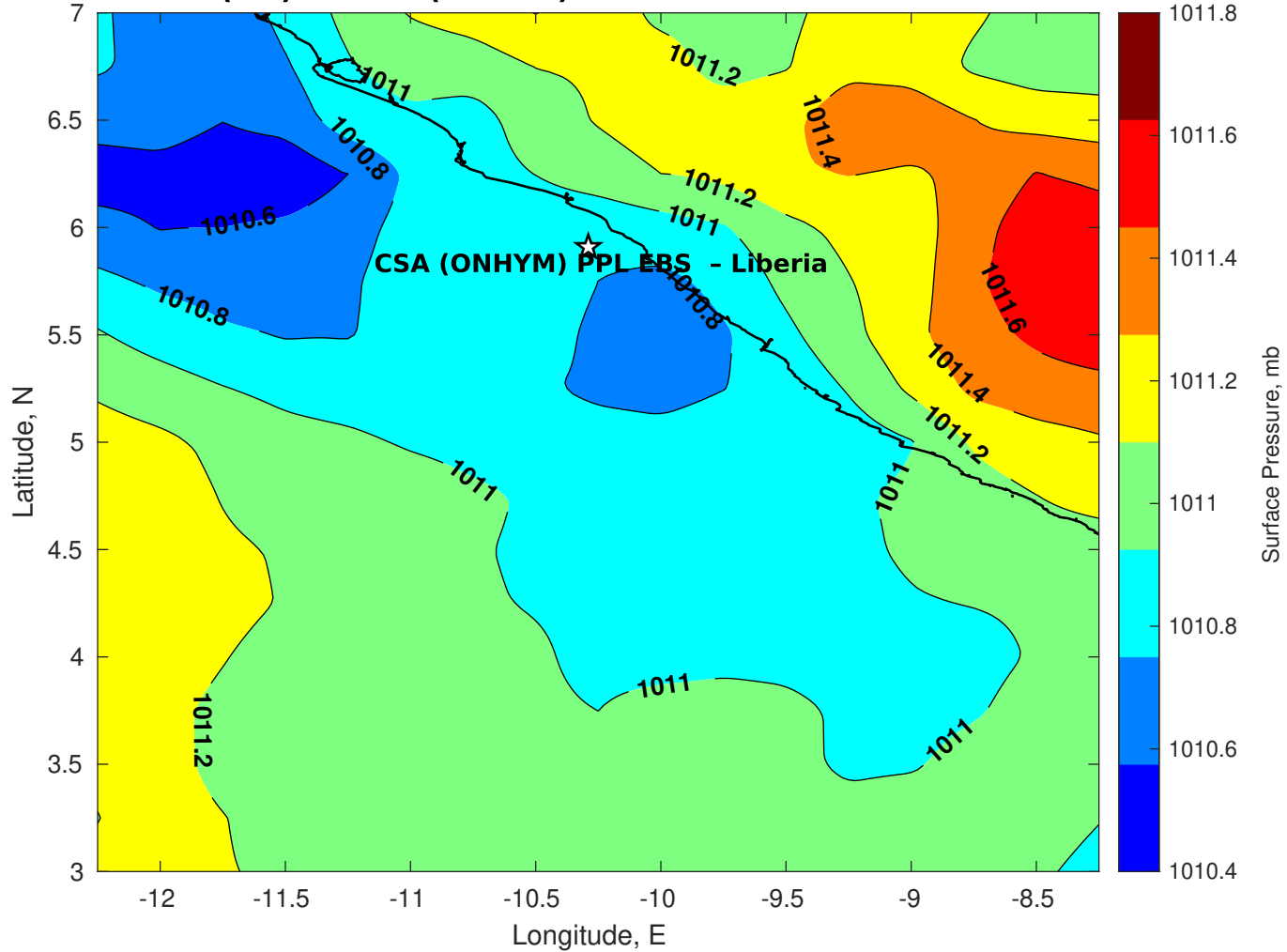
Surface Pressure (mb) for CSA (ONHYM) PPL EBS - Liberia at 08-Mar-2025 00:00:00
