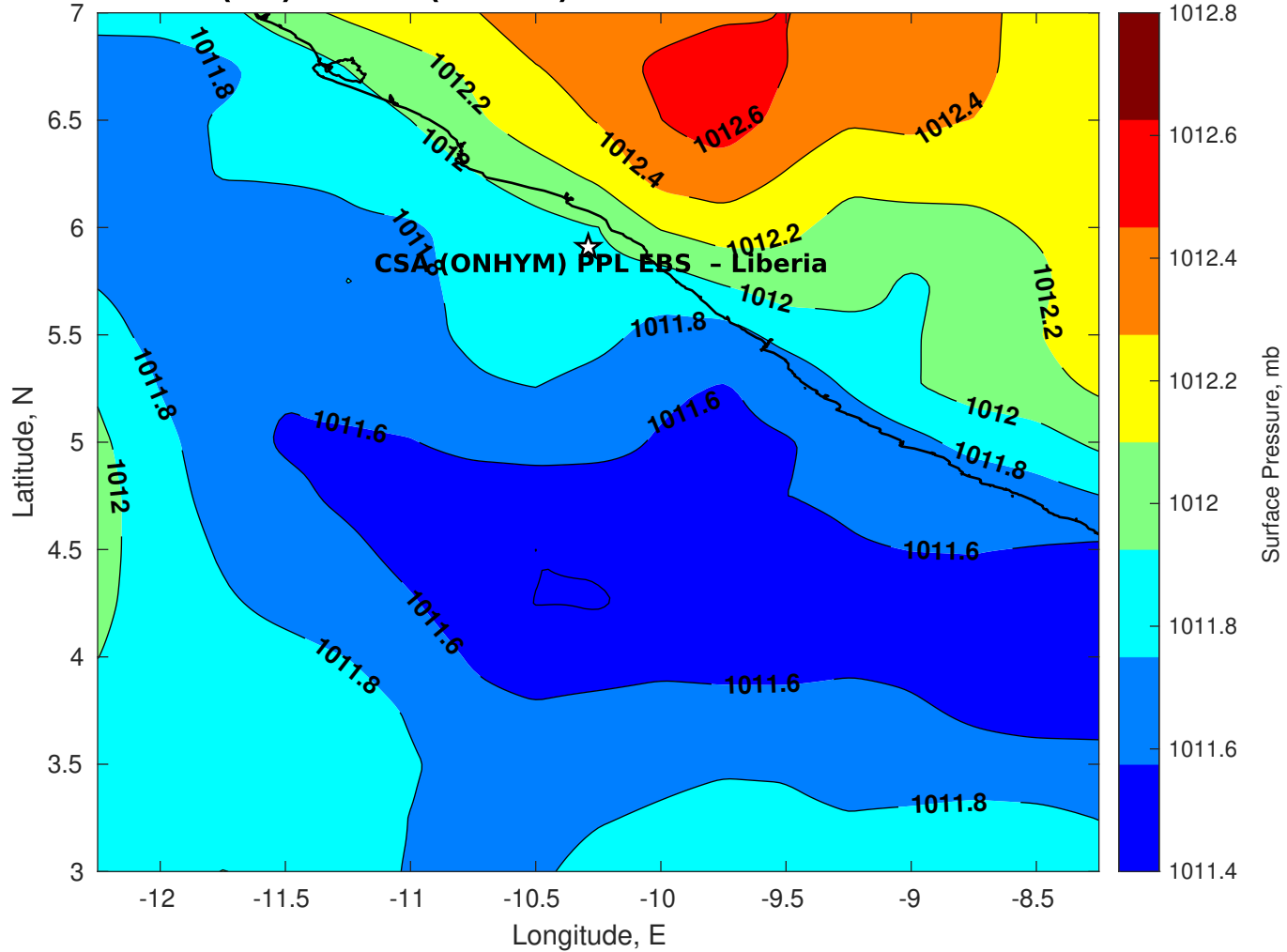
Surface Pressure (mb) for CSA (ONHYM) PPL EBS - Liberia at 07-Mar-2025 00:00:00
