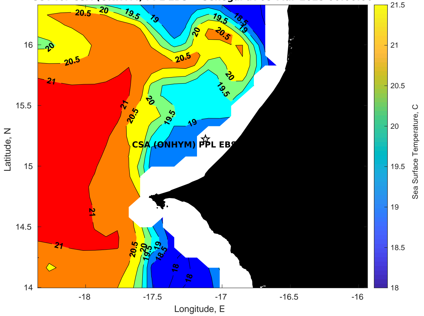
SST for CSA (ONHYM) PPL EBS - Senegal at 05-Mar-2025 00:00:00
