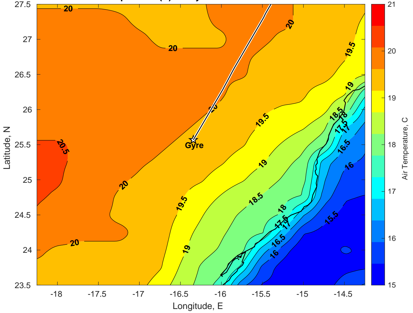
Air Temperature (C) for Gyre at 06-Mar-2025
