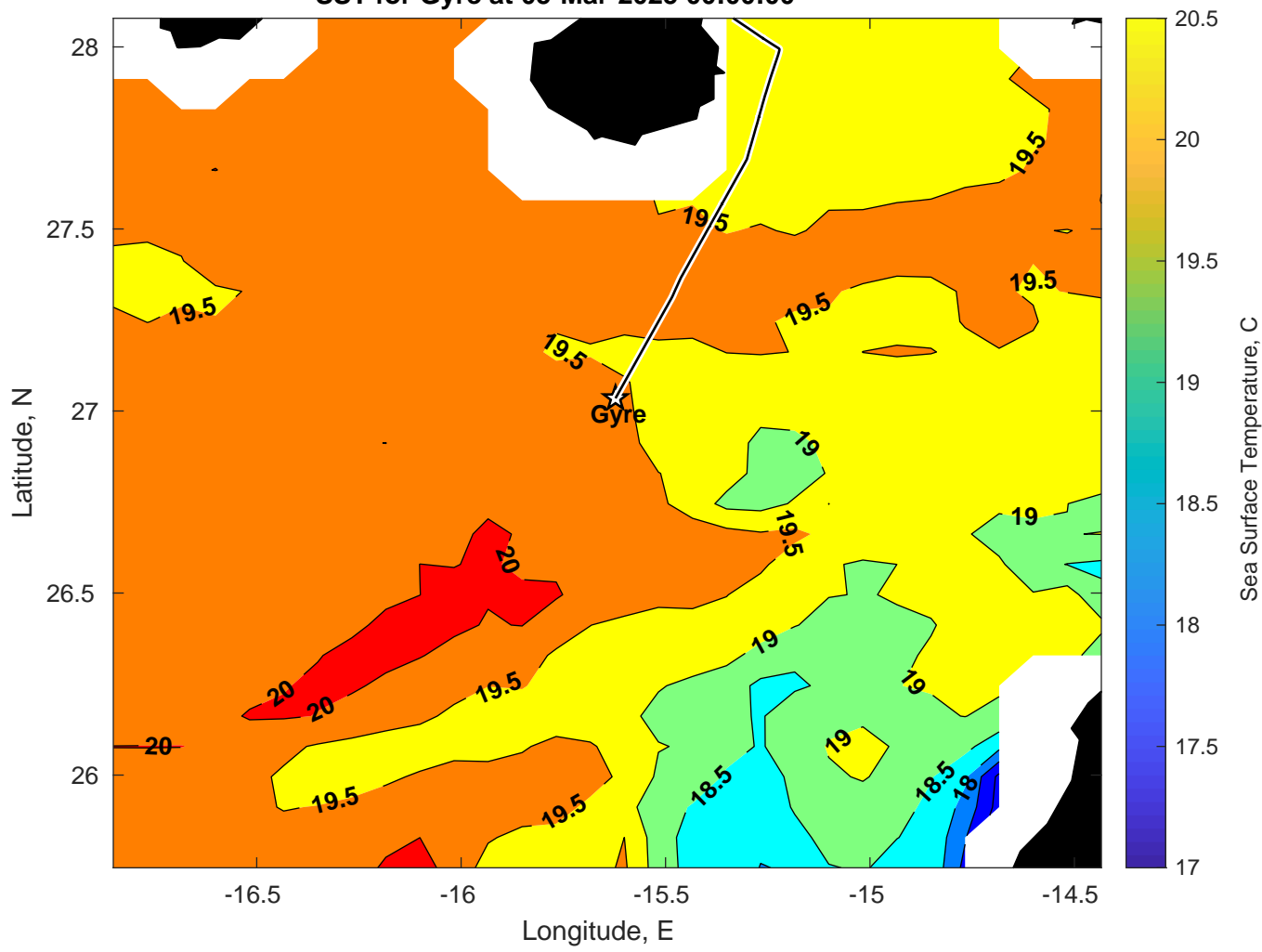
SST for Gyre at 05-Mar-2025 00:00:00
