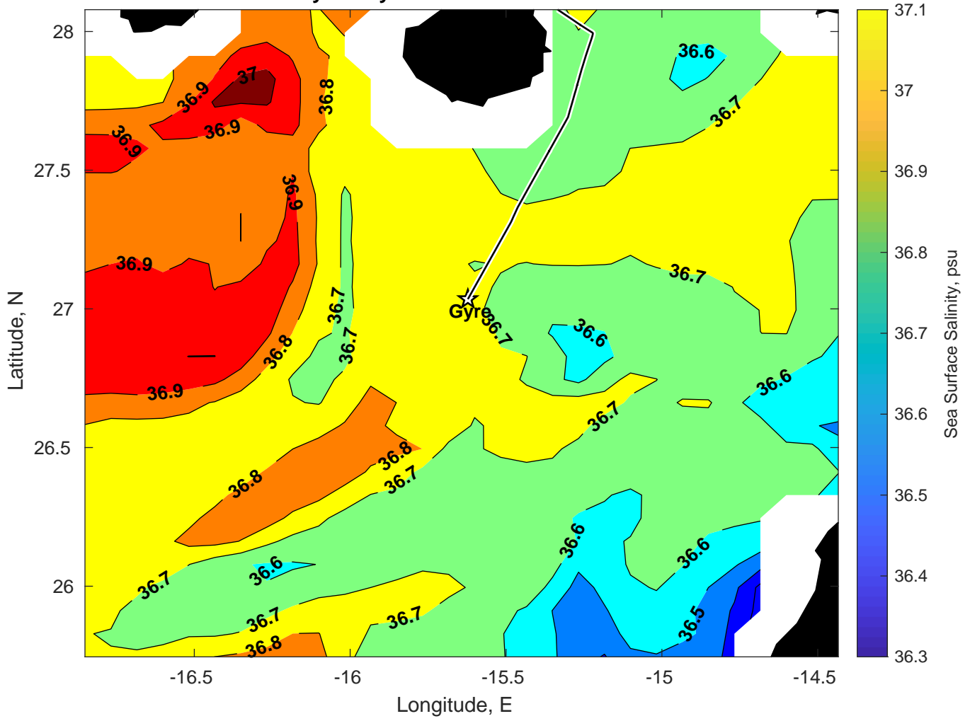
Surface Salinity for Gyre at 05-Mar-2025 00:00:00
