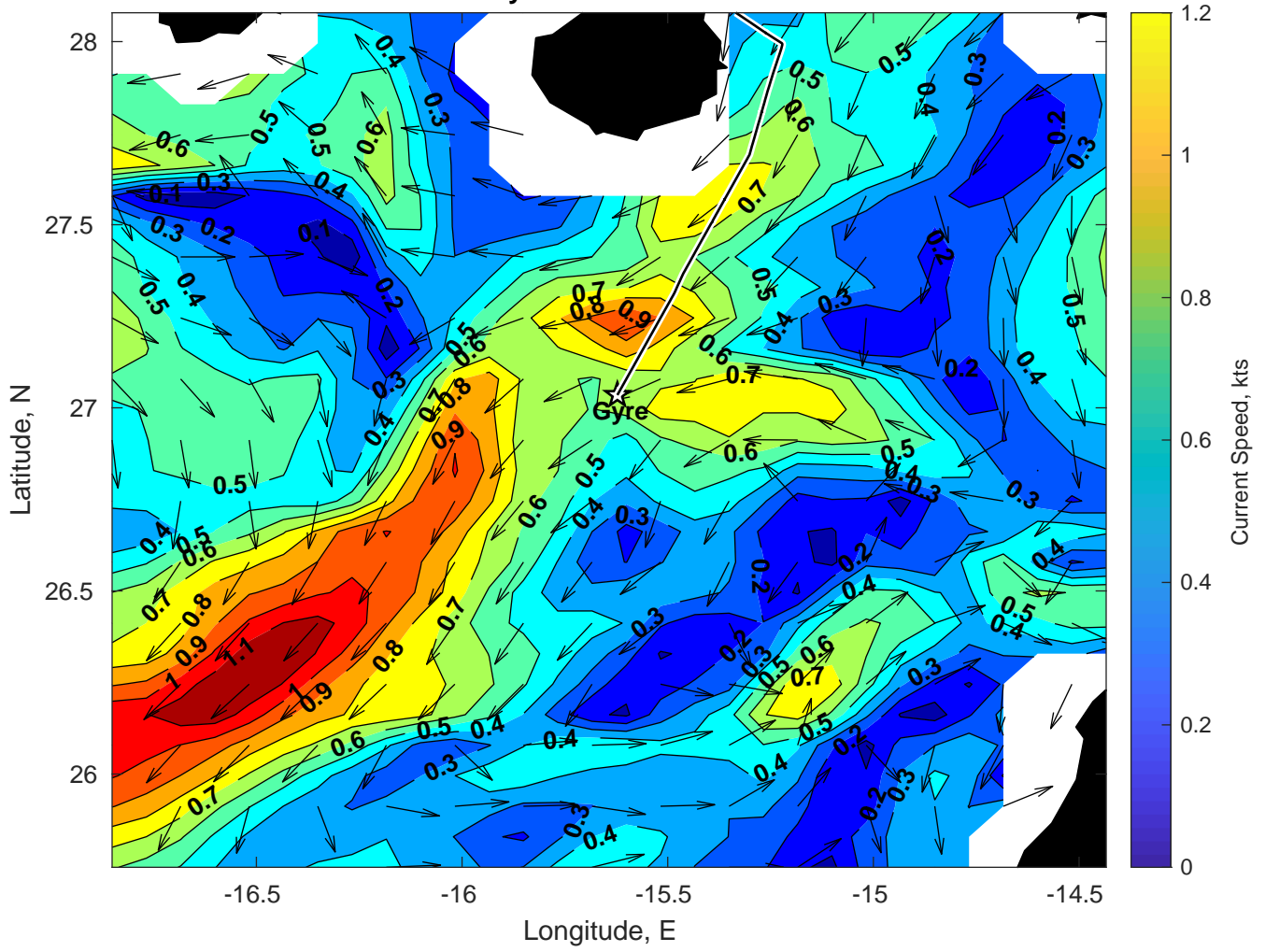
Surface Currents for Gyre at 05-Mar-2025 00:00:00
