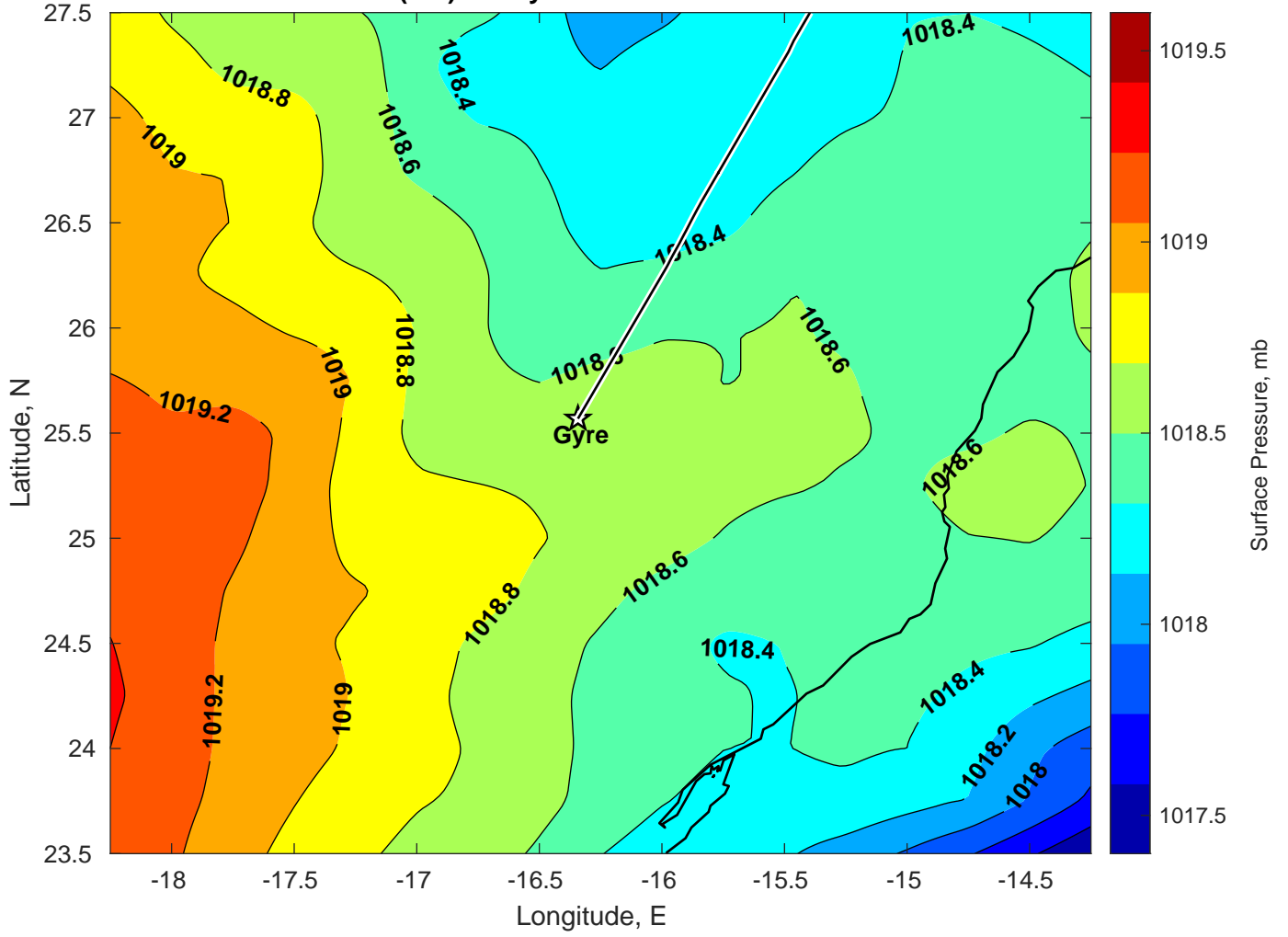
Surface Pressure (mb) for Gyre at 07-Mar-2025 00:00:00
