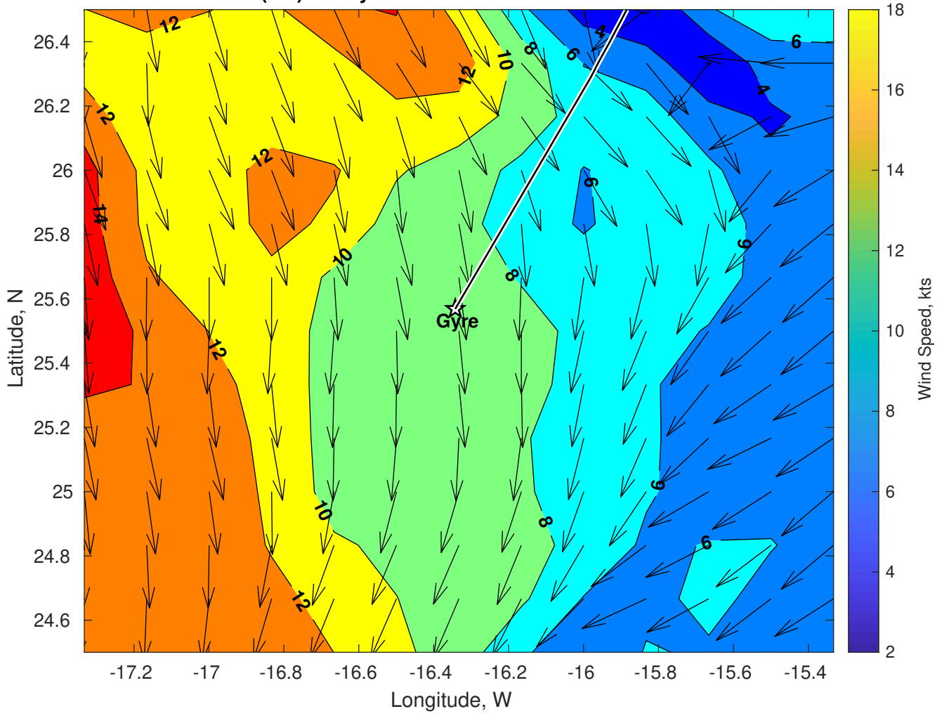
Winds (kts) for Gyre at 06-Mar-2025 09:00:00
