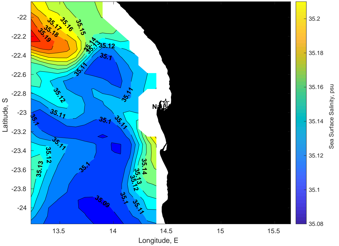
Surface Salinity for Nautilus at 05-Mar-2025 00:00:00
