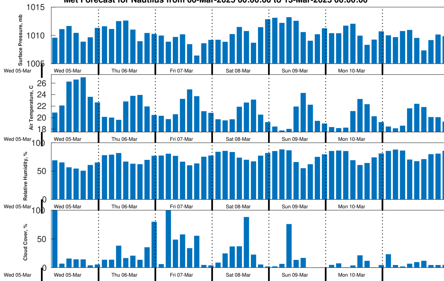
Met Forecast for Nautilus from 06-Mar-2025 00:00:00 to 13-Mar-2025 00:00:00
