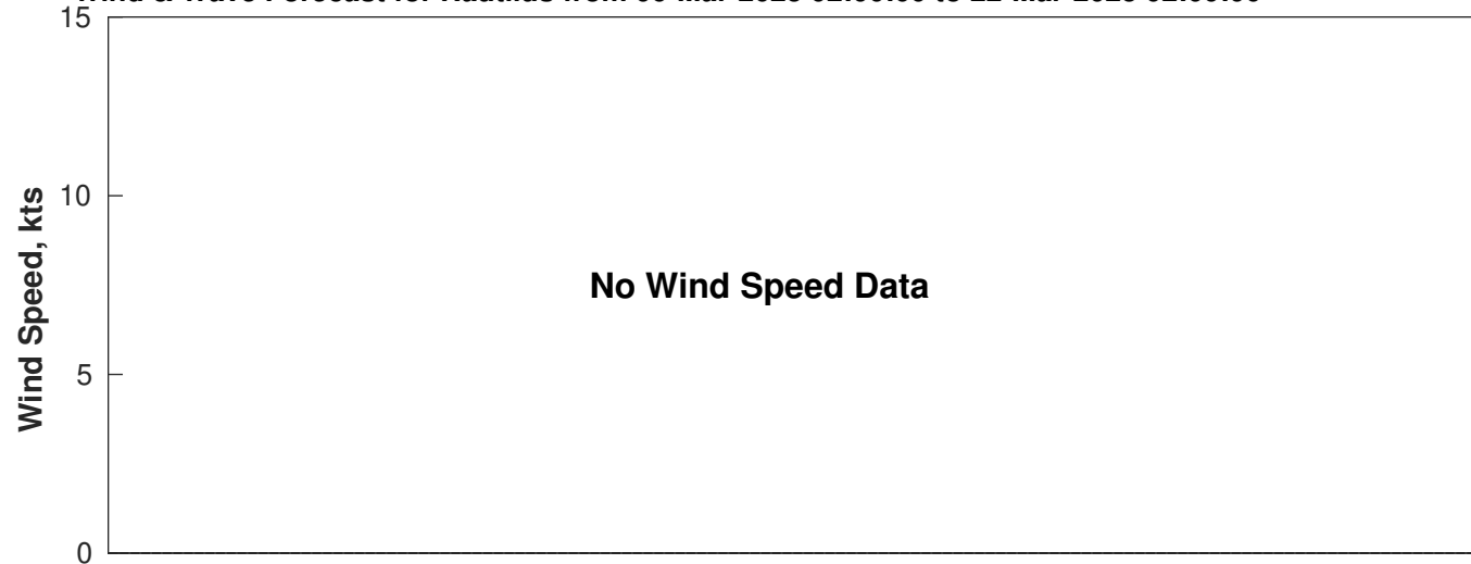
Wind & Wave Forecast for Nautilus from 06-Mar-2025 02:00:00 to 22-Mar-2025 02:00:00
