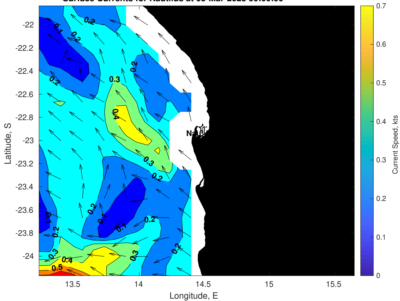
Surface Currents for Nautilus at 05-Mar-2025 00:00:00
