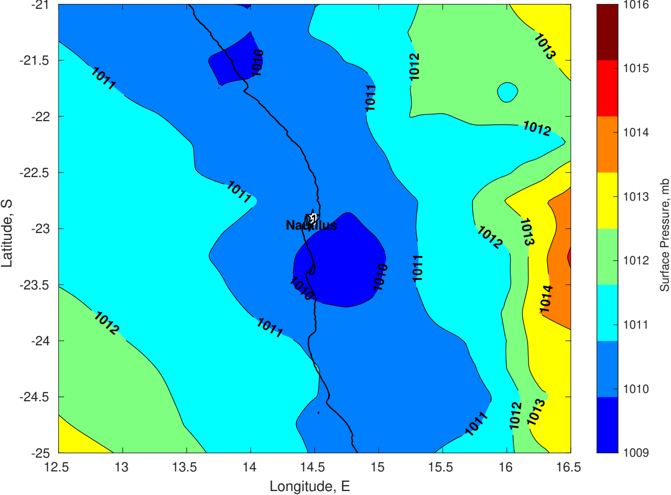
Surface Pressure (mb) for Nautilus at 06-Mar-2025 00:00:00
