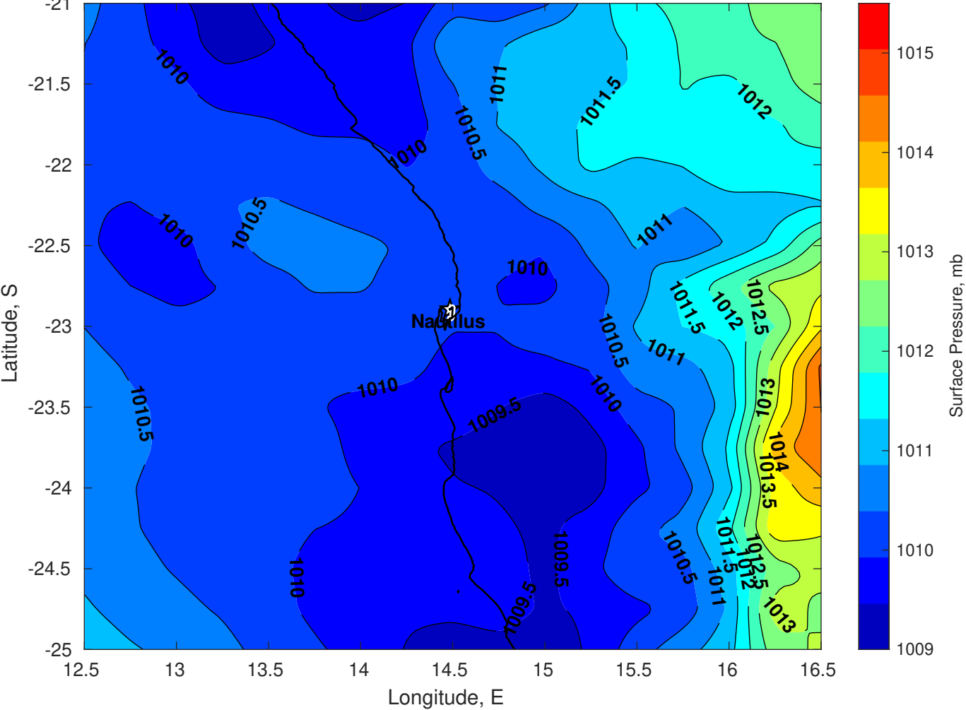
Surface Pressure (mb) for Nautilus at 08-Mar-2025 00:00:00
