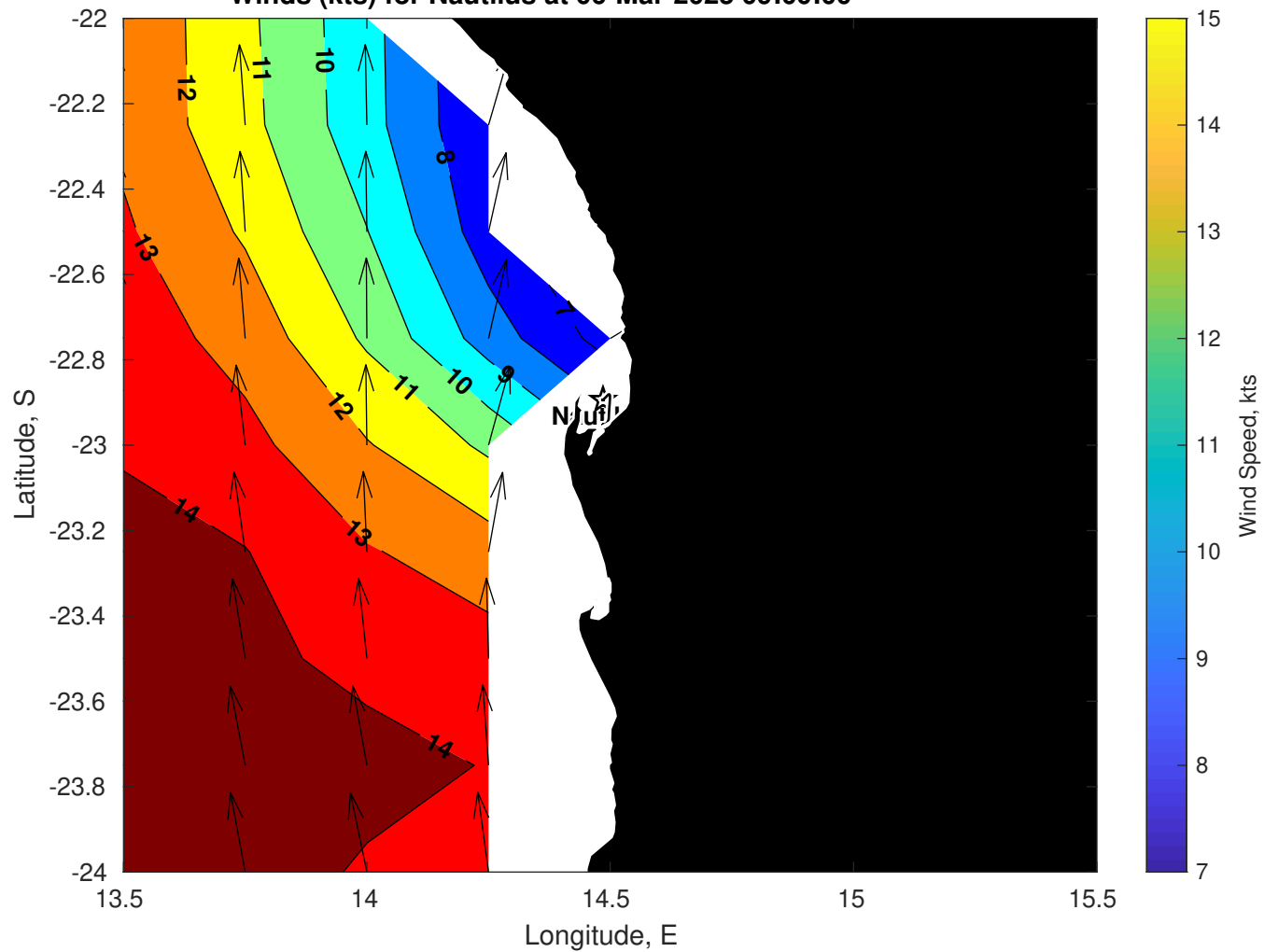
Winds (kts) for Nautilus at 06-Mar-2025 09:00:00
