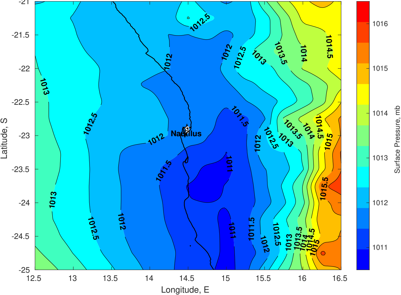
Surface Pressure (mb) for Nautilus at 07-Mar-2025 00:00:00
