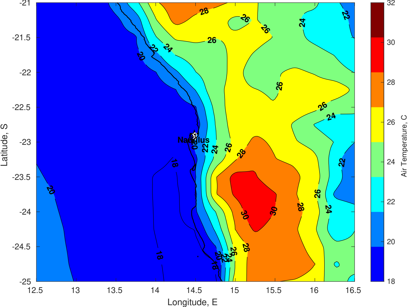
Air Temperature (C) for Nautilus at 06-Mar-2025
