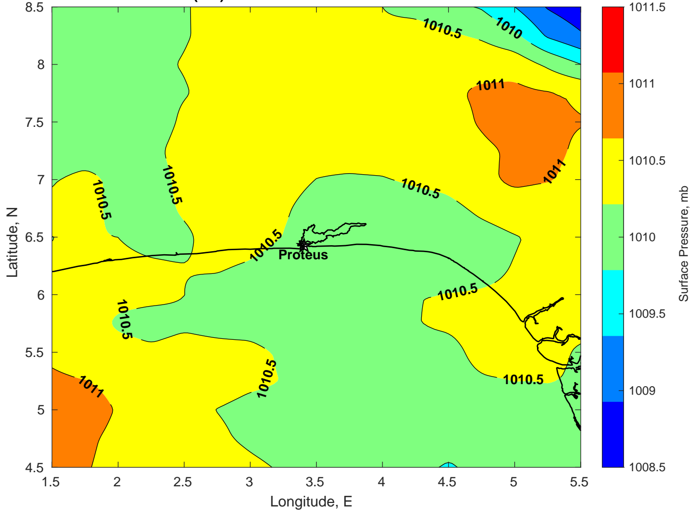
Surface Pressure (mb) for Proteus at 07-Mar-2025 00:00:00
