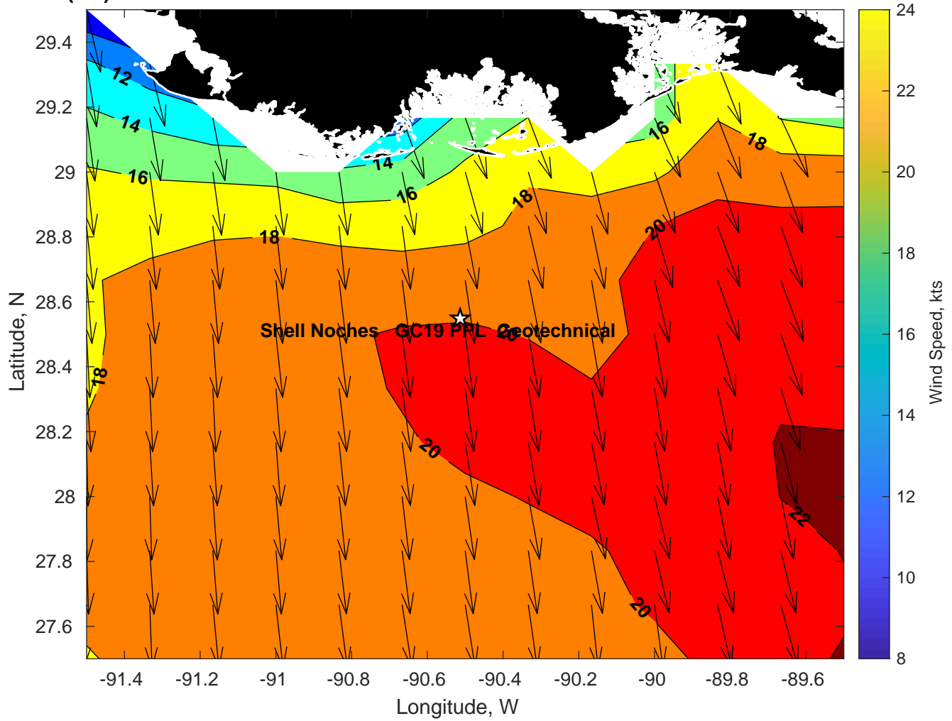
Winds (kts) for Shell Noches GC19 PPL Geotechnical at 06-Mar-2025 09:00:00
