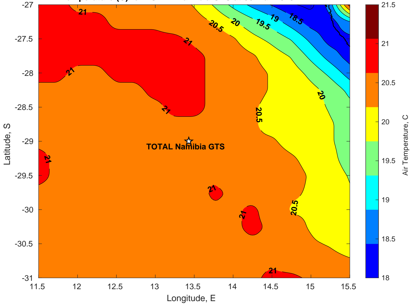
Air Temperature (C) for TOTAL Namibia GTS at 06-Mar-2025
