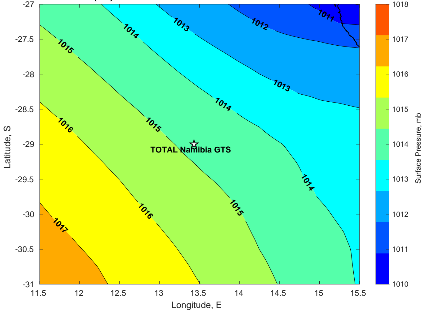
Surface Pressure (mb) for TOTAL Namibia GTS at 08-Mar-2025 00:00:00
