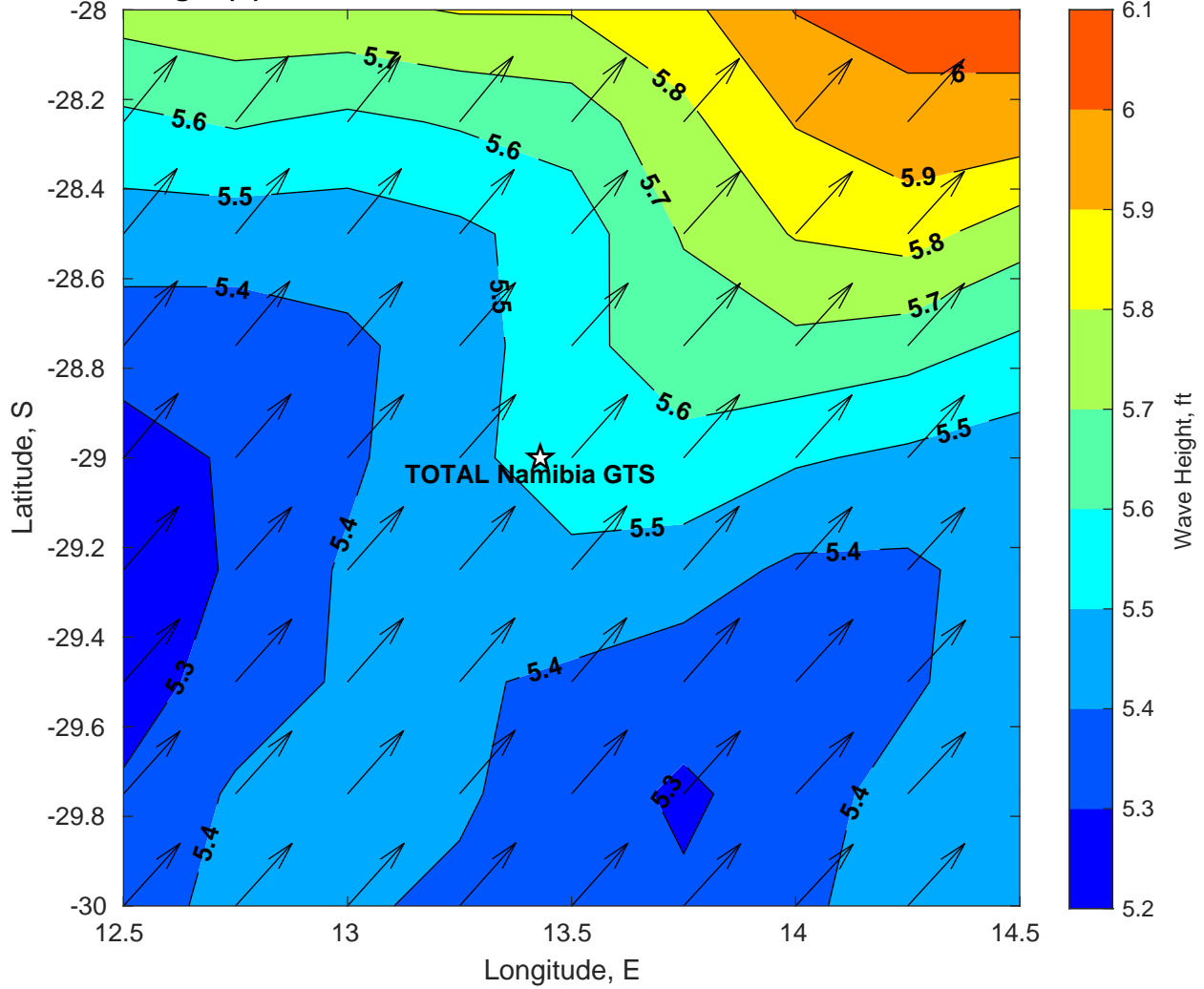
Wave Height (ft) for TOTAL Namibia GTS at 06-Mar-2025 09:00:00
