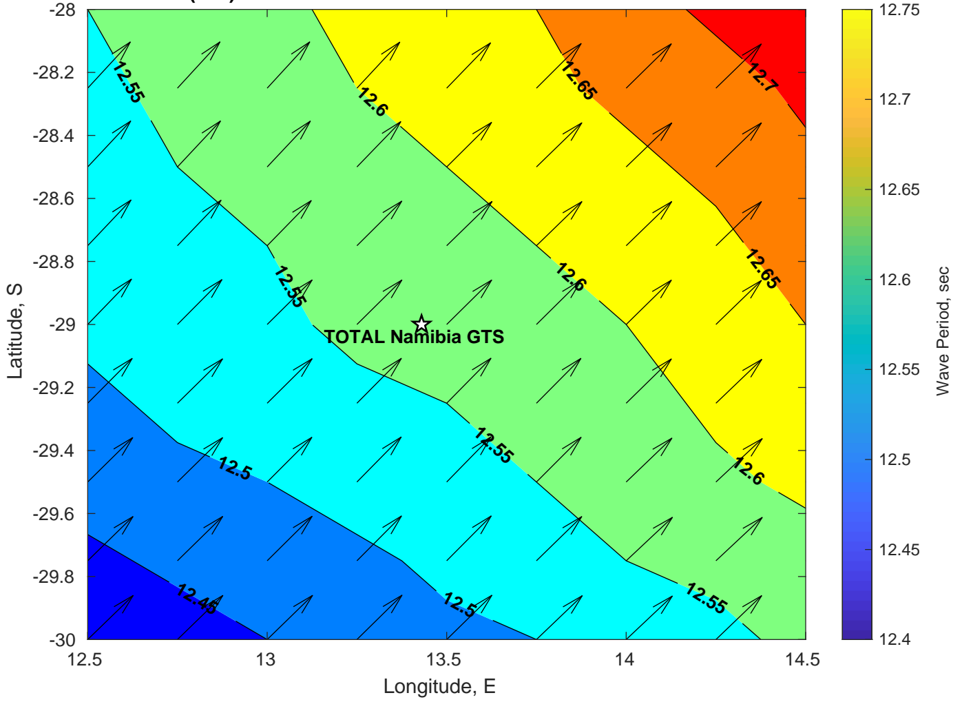
Wave Period (sec) for TOTAL Namibia GTS at 06-Mar-2025 09:00:00
