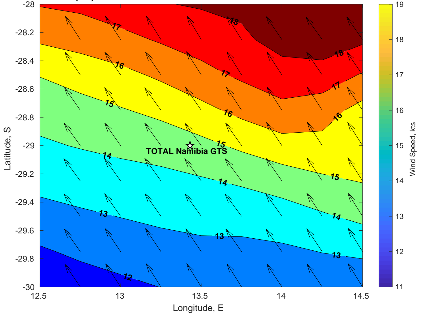
Winds (kts) for TOTAL Namibia GTS at 06-Mar-2025 09:00:00
