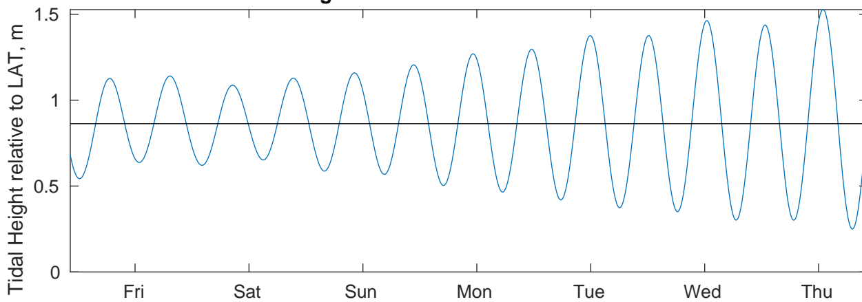
Tidal Currents and Heights for TOTAL Namibia GTS at 20250306
