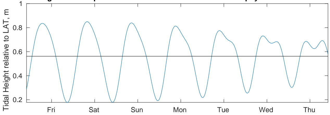
Tidal Currents and Heights for Tampnet P2378 South Texas Cable Route Geophysical at 20250306
