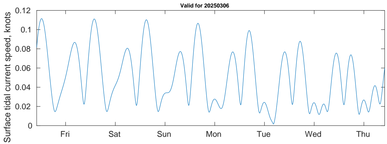
Tidal Currents and Heights for Tampnet P2378 South Texas Cable Route Geophysical at 20250306
