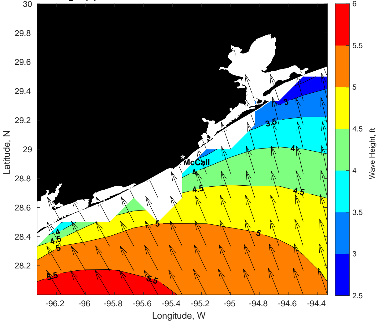
Wave Height (ft) for Brooks McCall at 07-Mar-2025 09:00:00
