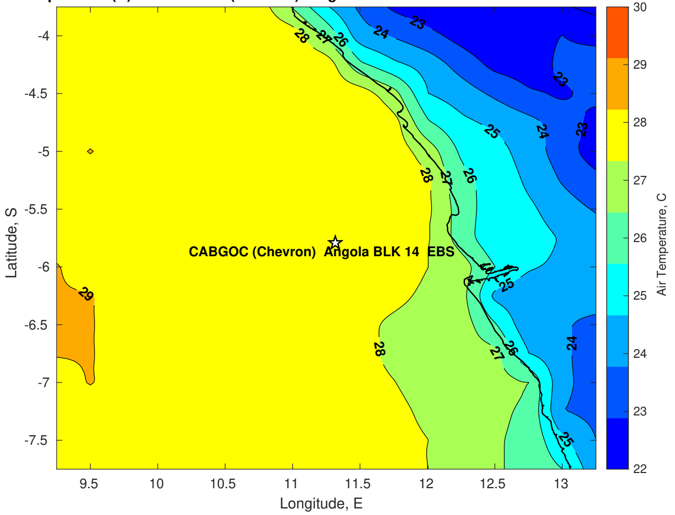
Air Temperature (C) for CABGOC (Chevron) Angola BLK 14 EBS at 07-Mar-2025
