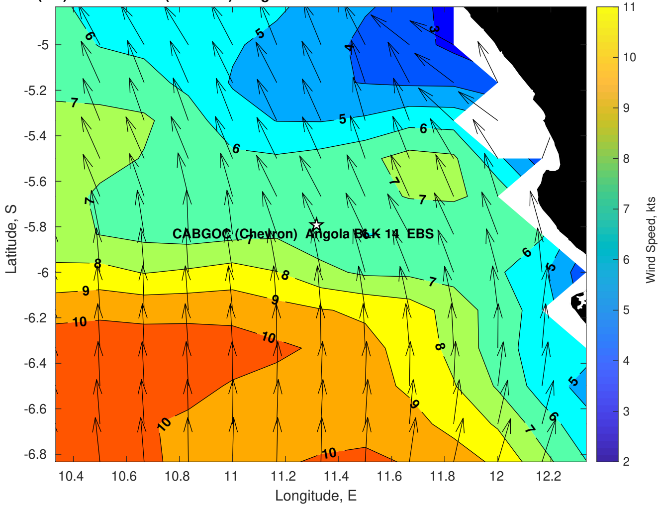
Winds (kts) for CABGOC (Chevron) Angola BLK 14 EBS at 07-Mar-2025 09:00:00
