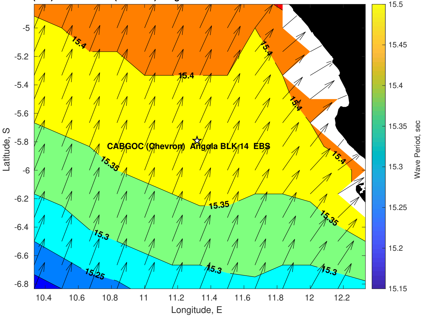
Wave Period (sec) for CABGOC (Chevron) Angola BLK 14 EBS at 07-Mar-2025 09:00:00
