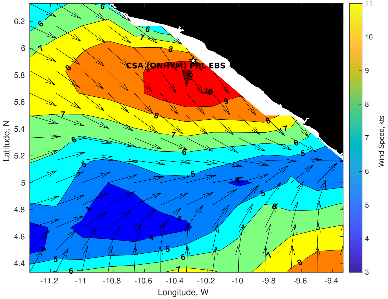
Winds (kts) for CSA (ONHYM) PPL EBS - Liberia at 07-Mar-2025 09:00:00
