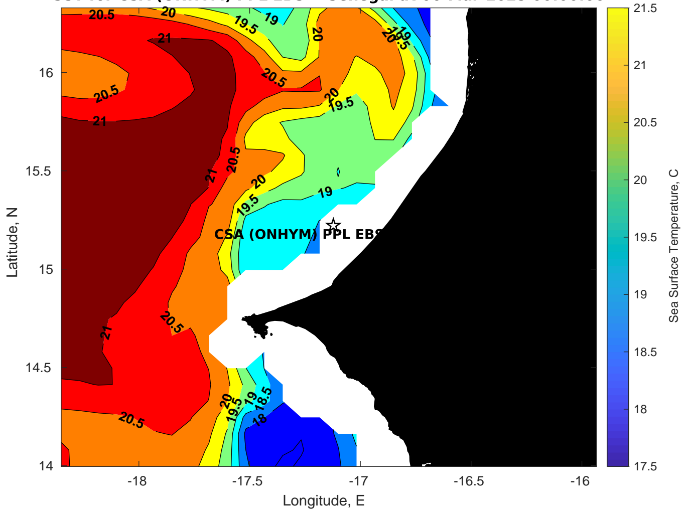
SST for CSA (ONHYM) PPL EBS - Senegal at 06-Mar-2025 00:00:00
