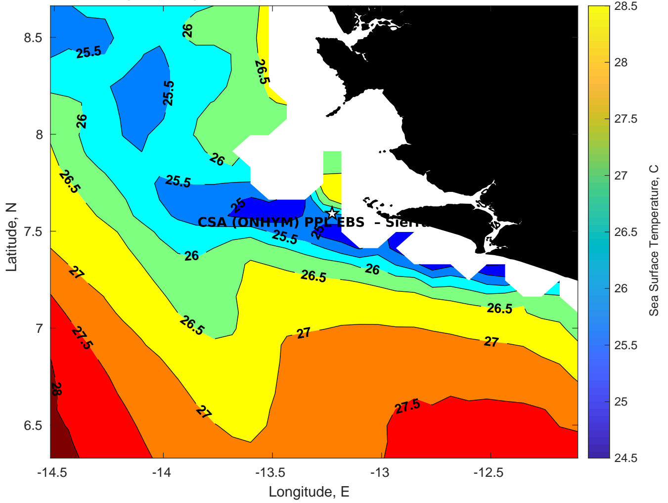
SST for CSA (ONHYM) PPL EBS - Sierra Leone at 06-Mar-2025 00:00:00
