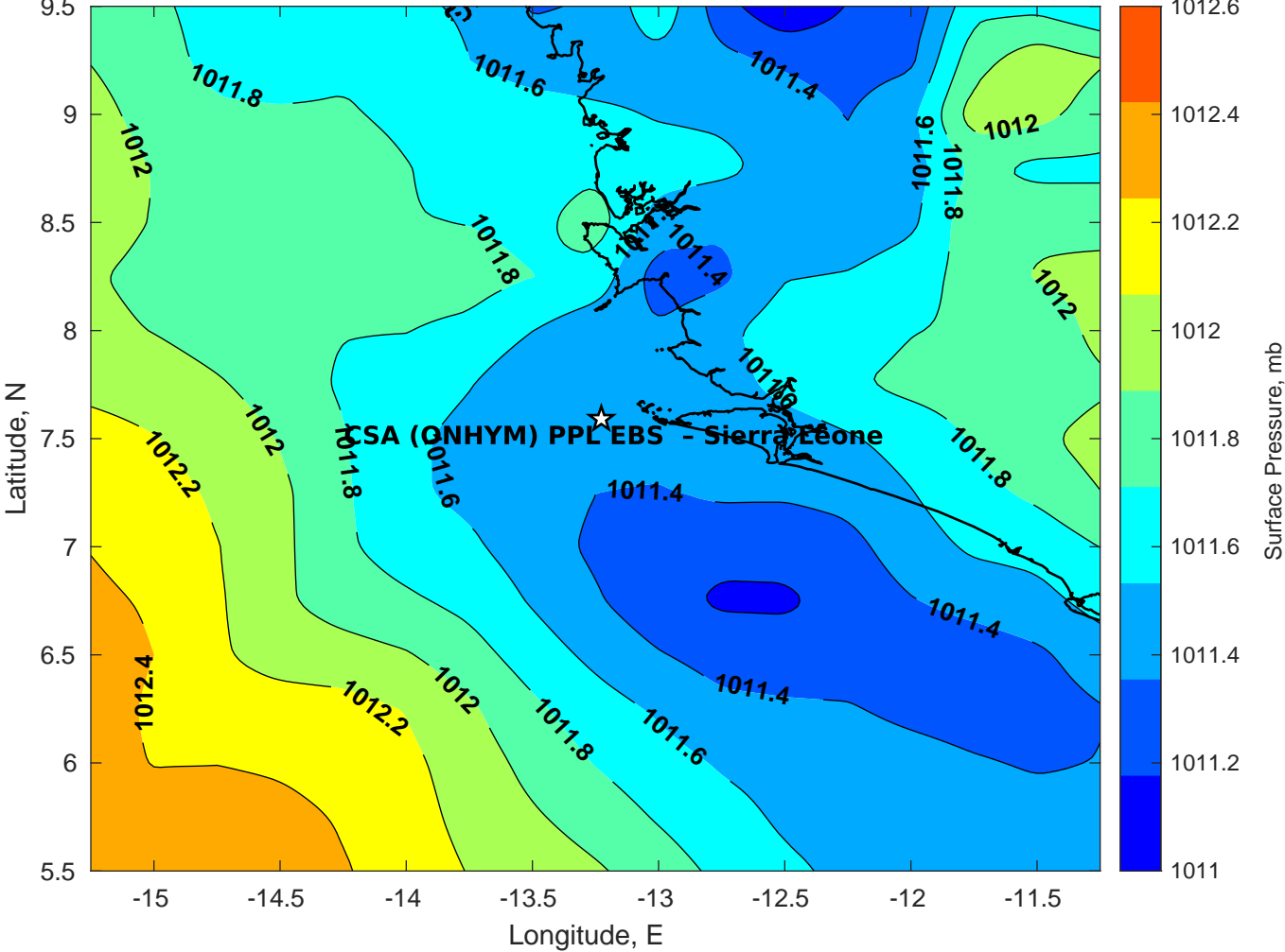
Surface Pressure (mb) for CSA (ONHYM) PPL EBS - Sierra Leone at 07-Mar-2025 00:00:00
