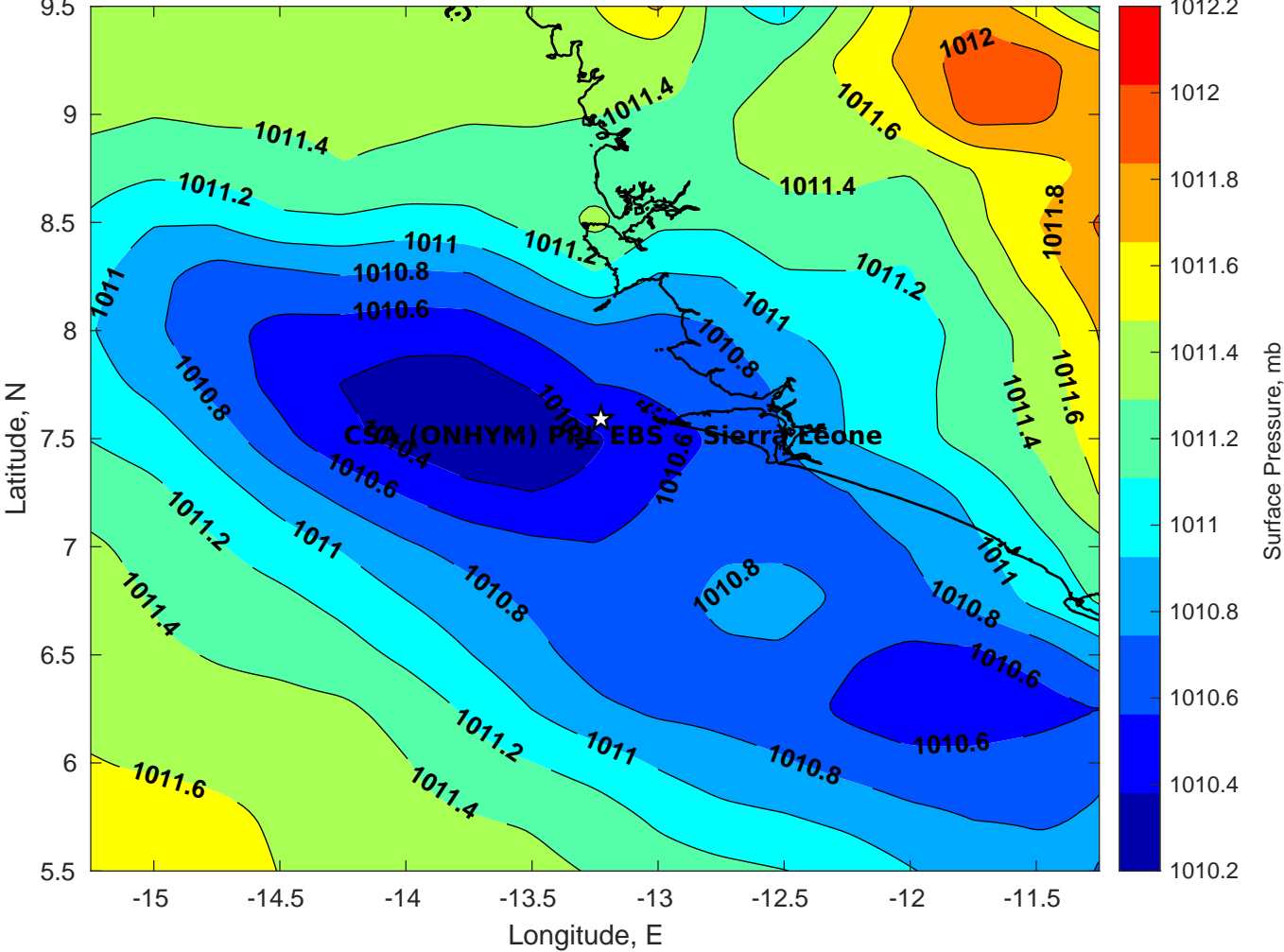
Surface Pressure (mb) for CSA (ONHYM) PPL EBS - Sierra Leone at 08-Mar-2025 00:00:00
