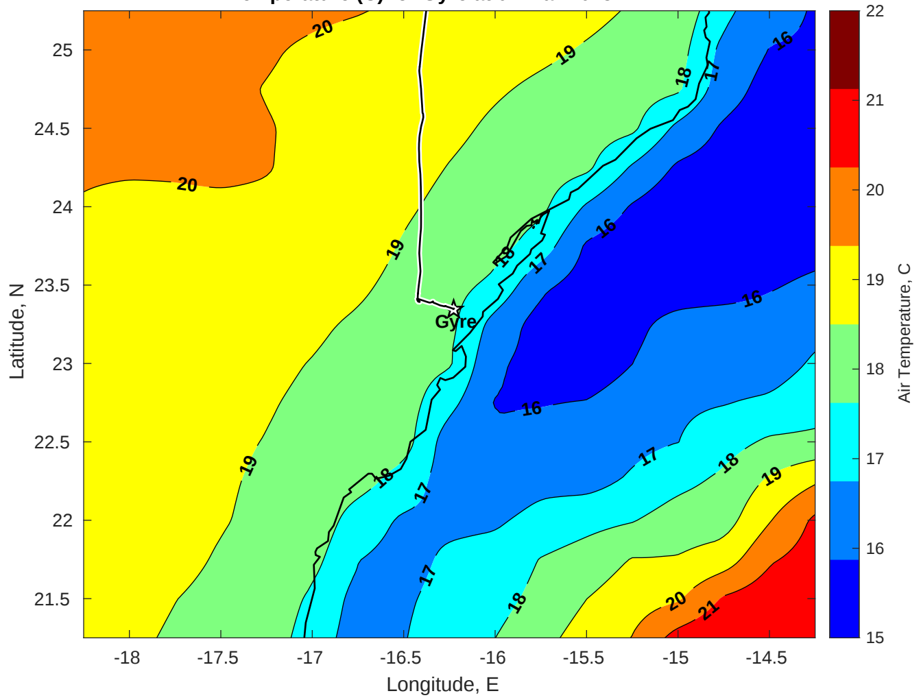
Air Temperature (C) for Gyre at 07-Mar-2025
