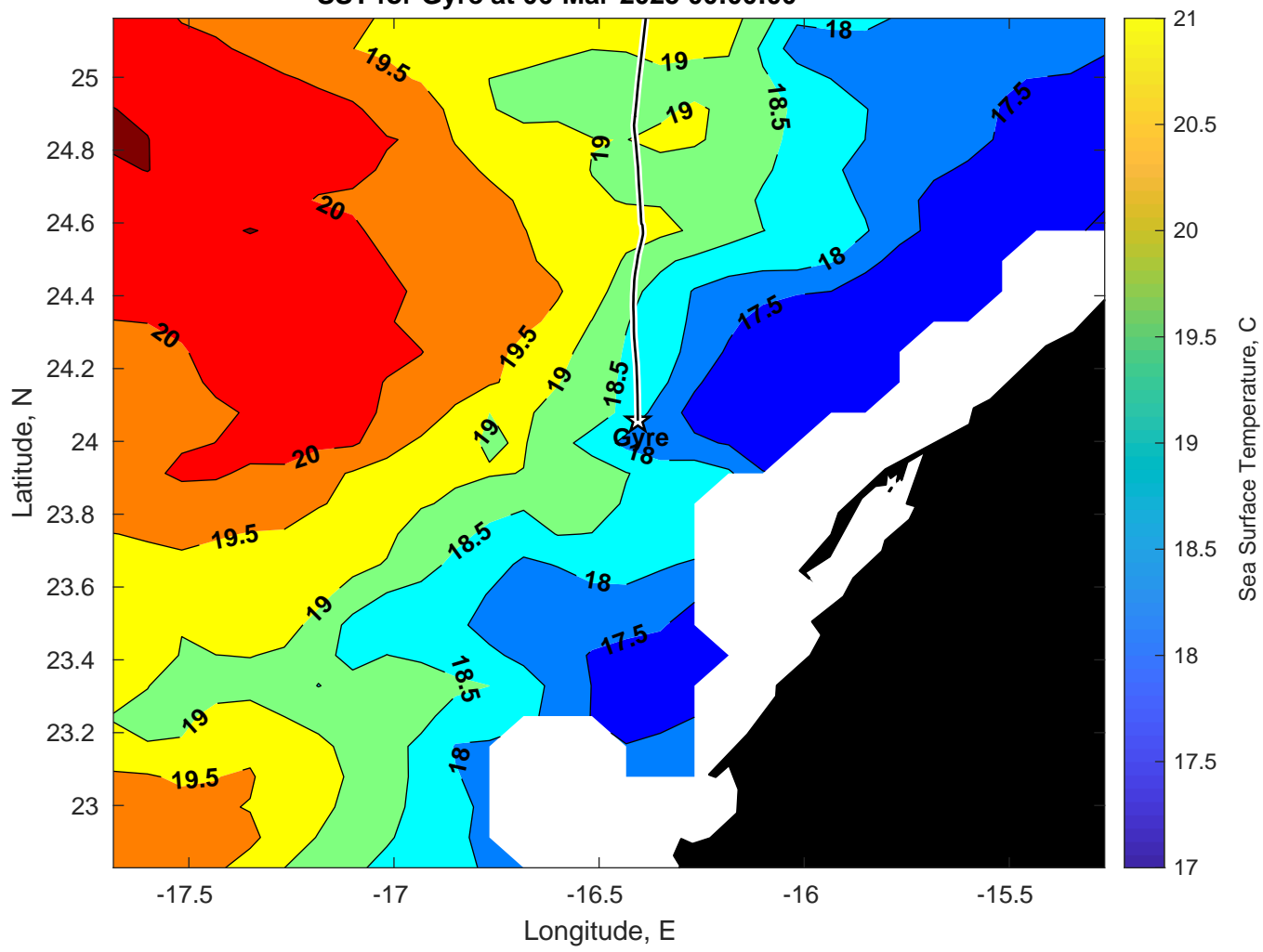
SST for Gyre at 06-Mar-2025 00:00:00
