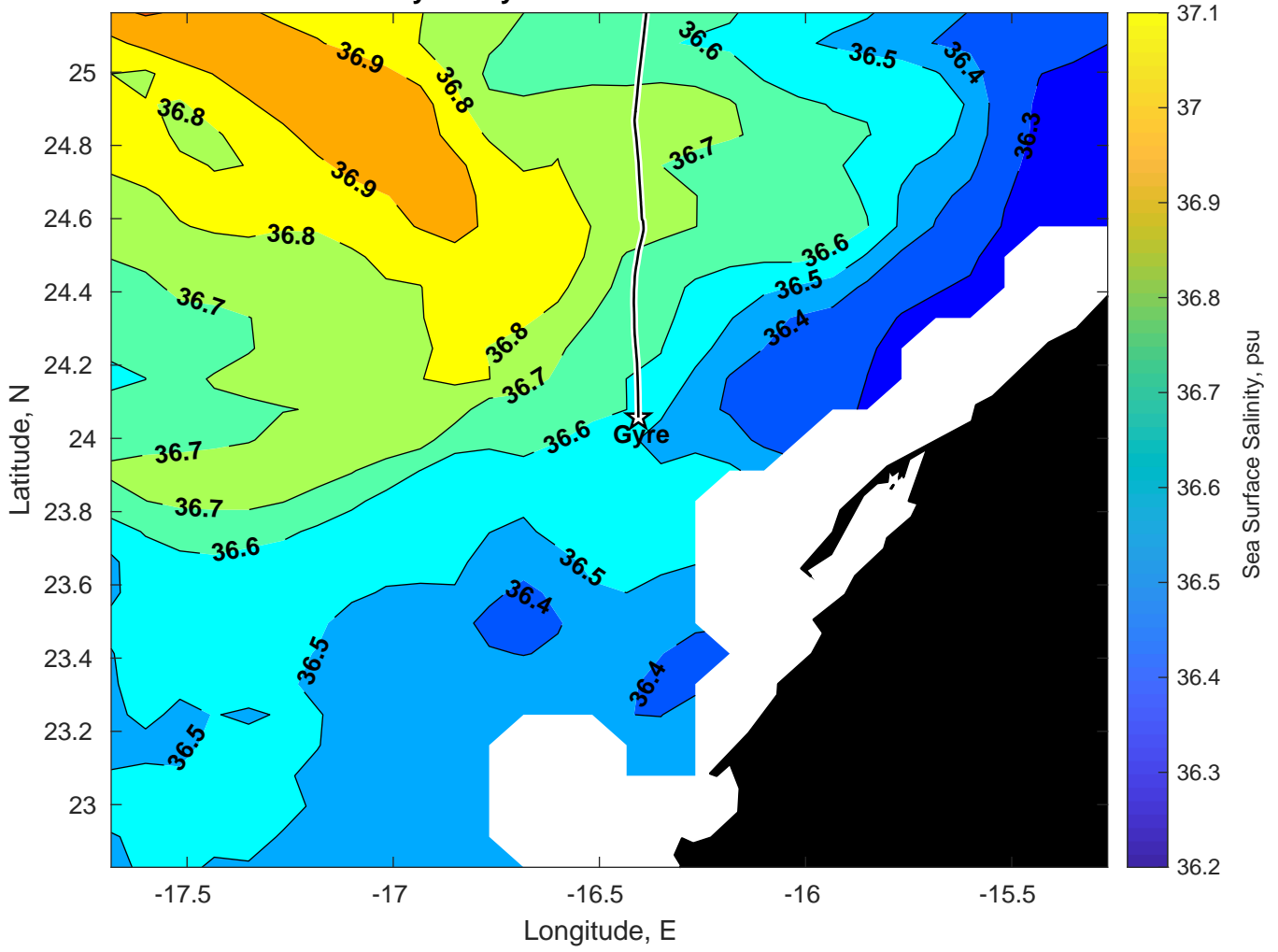
Surface Salinity for Gyre at 06-Mar-2025 00:00:00
