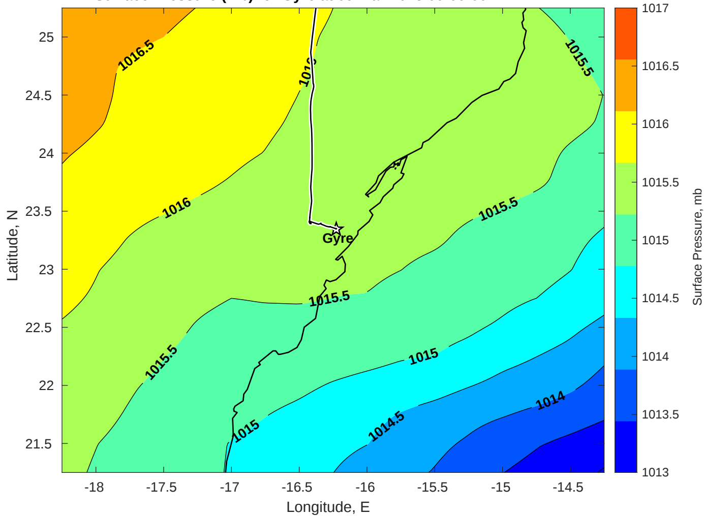
Surface Pressure (mb) for Gyre at 09-Mar-2025 00:00:00
