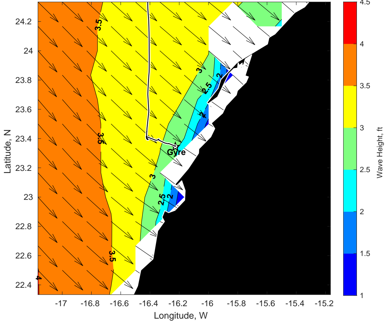
Wave Height (ft) for Gyre at 07-Mar-2025 09:00:00
