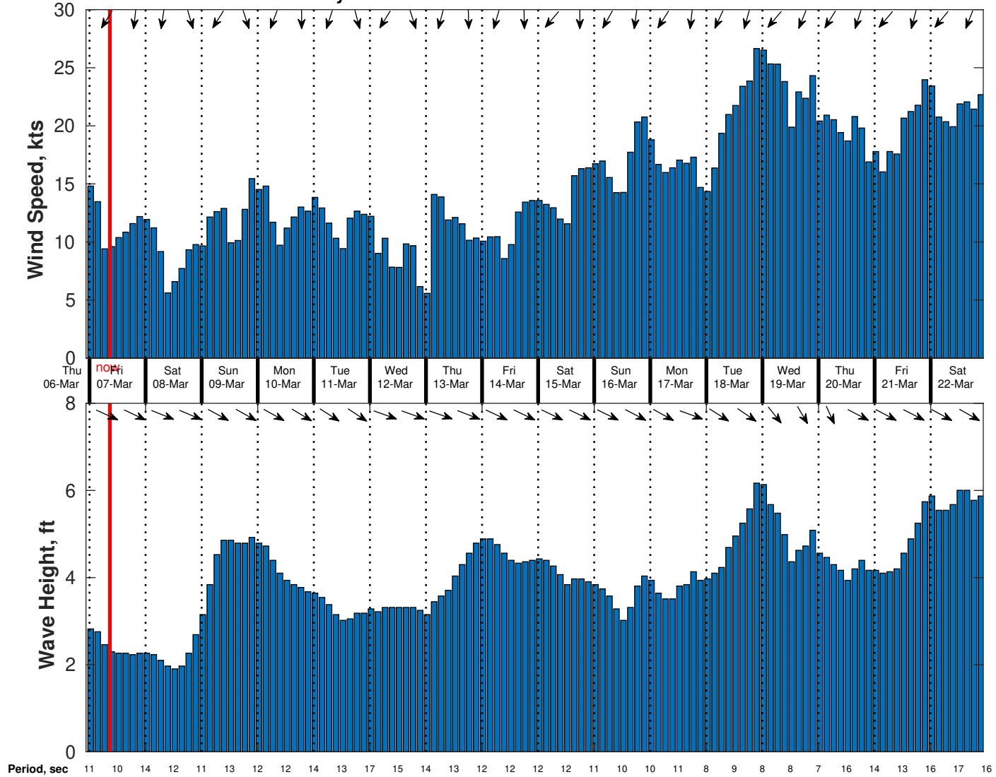
Wind & Wave Forecast for Gyre from 06-Mar-2025 23:00:00 to 22-Mar-2025 23:00:00
