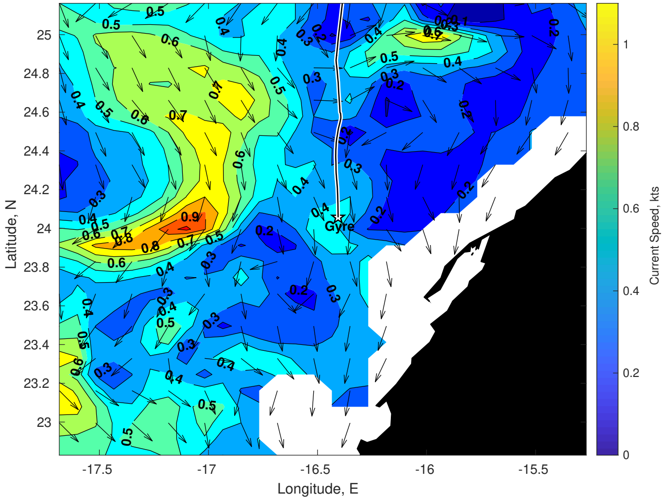
Surface Currents for Gyre at 06-Mar-2025 00:00:00
