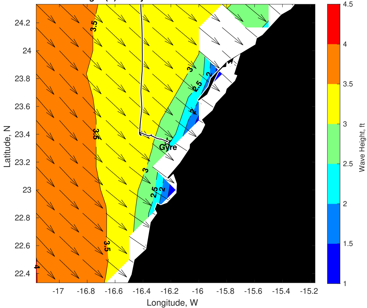
Wave Height (ft) for Gyre at 07-Mar-2025 09:00:00
