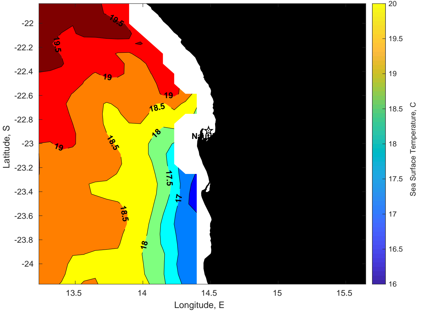
SST for Nautilus at 06-Mar-2025 00:00:00
