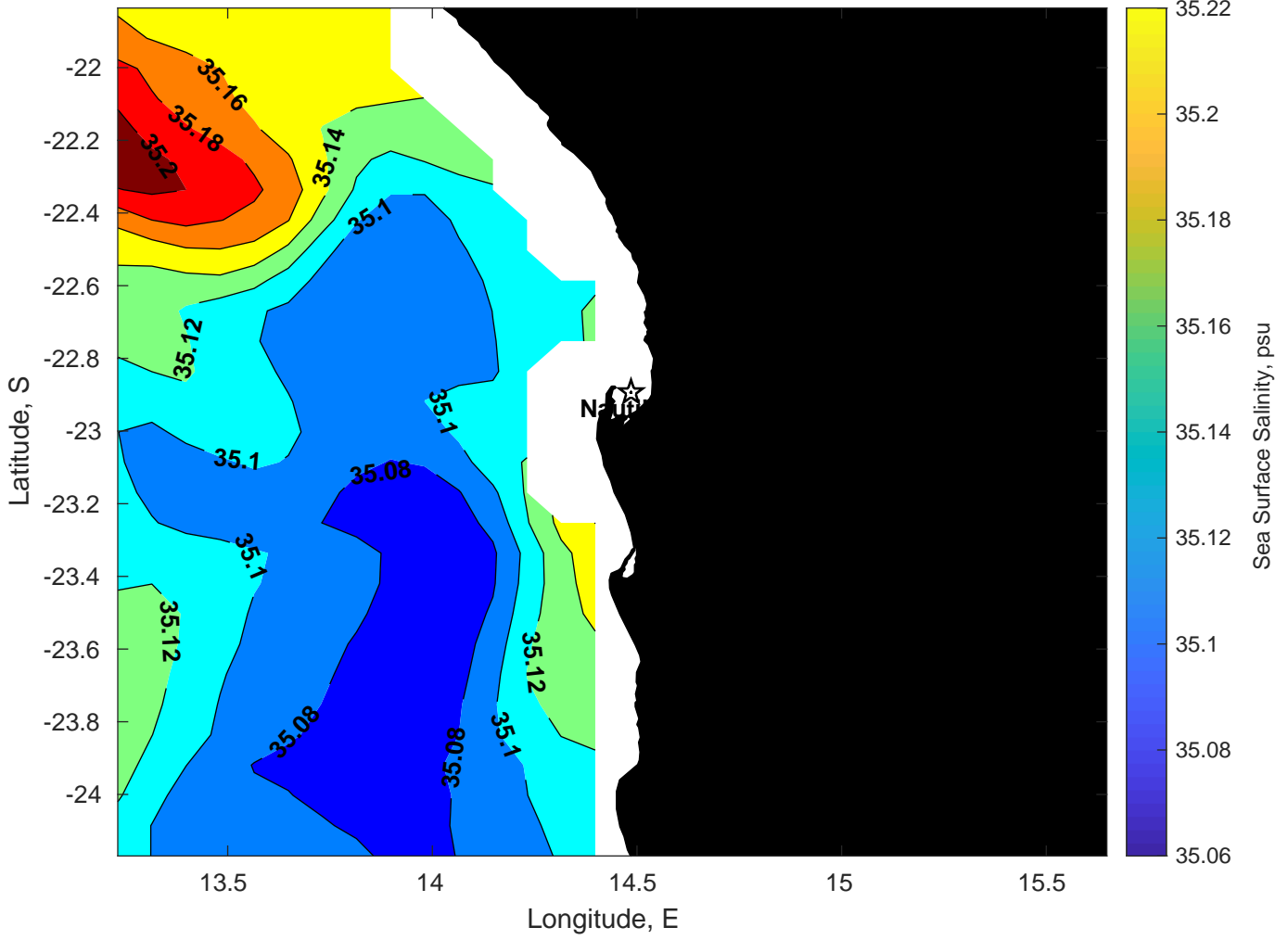
Surface Salinity for Nautilus at 06-Mar-2025 00:00:00
