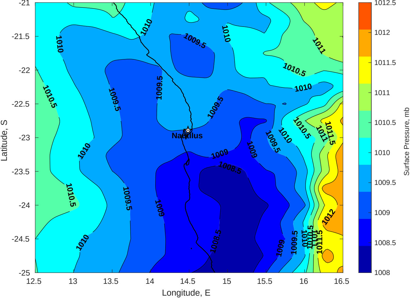
Surface Pressure (mb) for Nautilus at 09-Mar-2025 00:00:00
