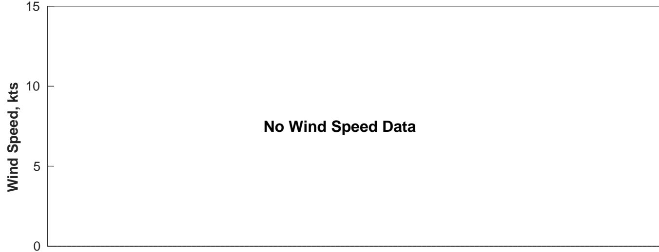
Wind & Wave Forecast for Nautilus from 07-Mar-2025 02:00:00 to 23-Mar-2025 02:00:00
